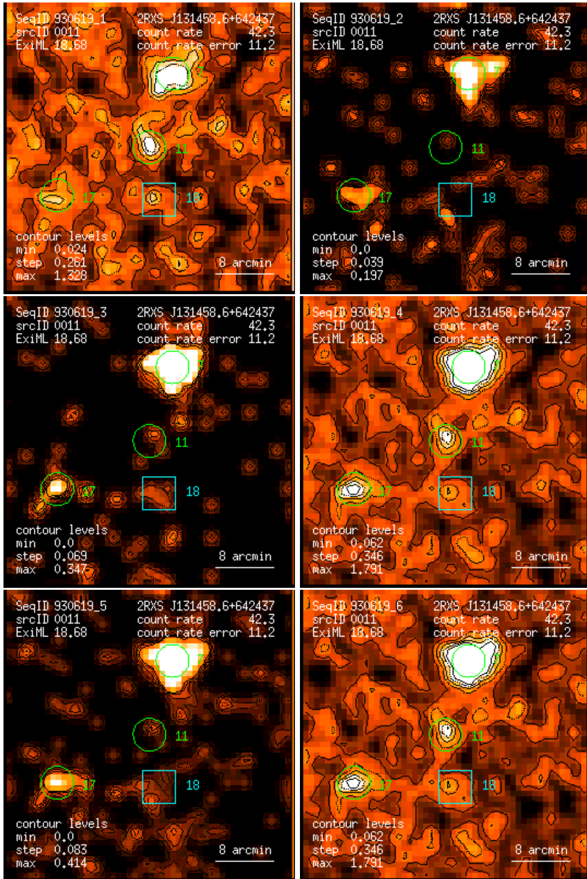
Figure 11: RASS 930619: detection 0011: band rate images, Gaussian filter: (1) PSPC channels 11 – 41, (2) 52 – 90, (3) 91 – 201, (4) 11 – 235, (5) 52 – 201, (6) 11 – 201. Broad band rates in counts/ks. Band rate contour levels in counts/ks/arcmin 2 .
