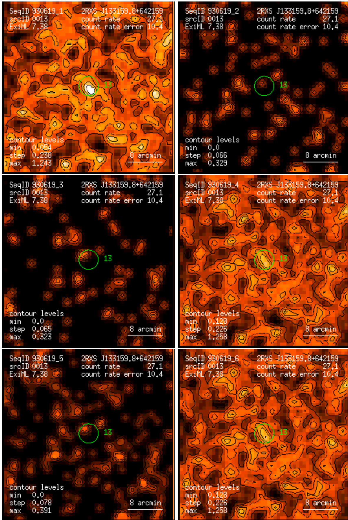
Figure 13: RASS 930619: detection 0013: band rate images, Gaussian filter: (1) PSPC channels 11 – 41, (2) 52 – 90, (3) 91 – 201, (4) 11 – 235, (5) 52 – 201, (6) 11 – 201. Broad band rates in counts/ks. Band rate contour levels in counts/ks/arcmin 2 .
