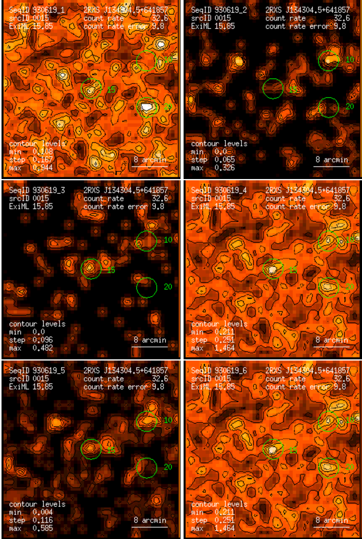
Figure 15: RASS 930619: detection 0015: band rate images, Gaussian filter: (1) PSPC channels 11 – 41, (2) 52 – 90, (3) 91 – 201, (4) 11 – 235, (5) 52 – 201, (6) 11 – 201. Broad band rates in counts/ks. Band rate contour levels in counts/ks/arcmin 2 .
