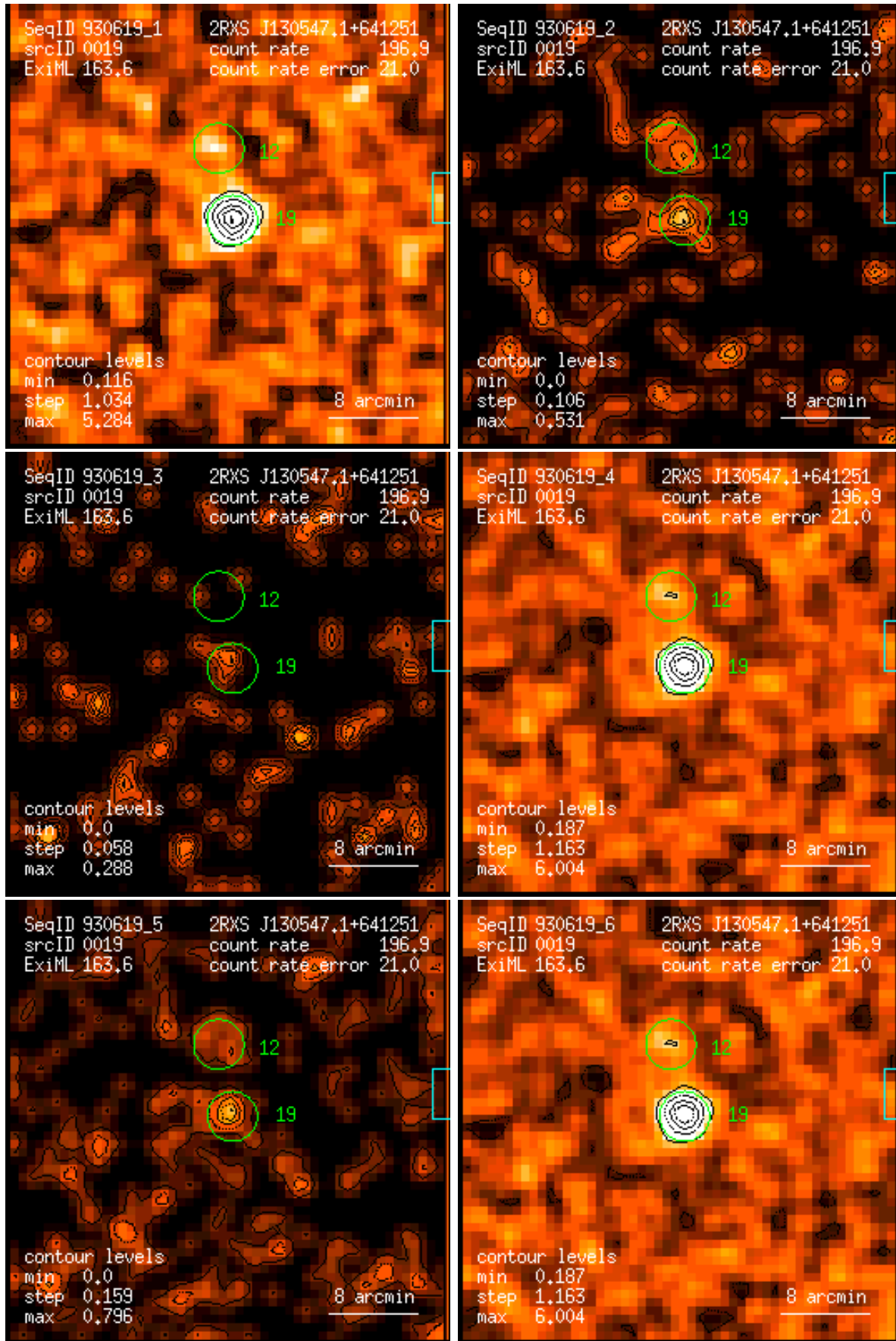
Figure 19: RASS 930619: detection 0019: band rate images, Gaussian filter: (1) PSPC channels 11 – 41, (2) 52 – 90, (3) 91 – 201, (4) 11 – 235, (5) 52 – 201, (6) 11 – 201. Broad band rates in counts/ks. Band rate contour levels in counts/ks/arcmin 2 .
