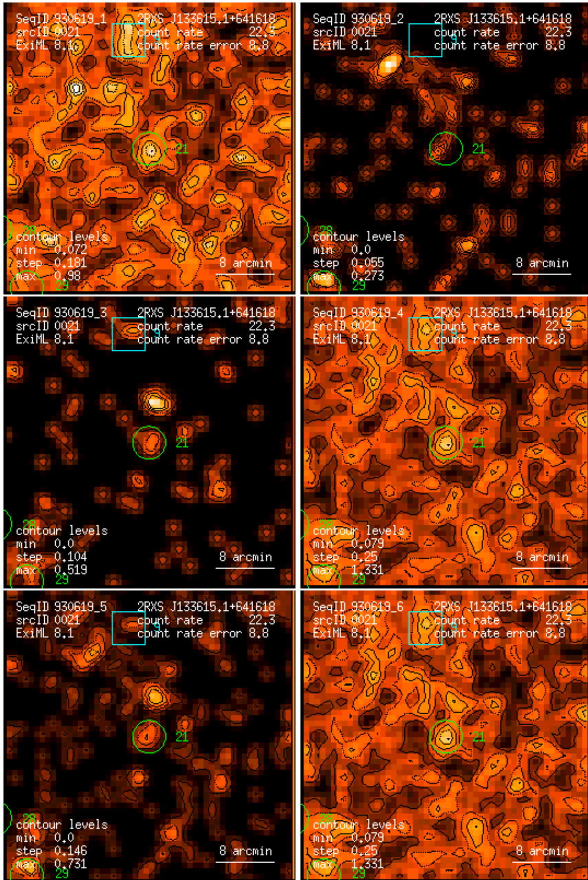
Figure 21: RASS 930619: detection 0021: band rate images, Gaussian filter: (1) PSPC channels 11 – 41, (2) 52 – 90, (3) 91 – 201, (4) 11 – 235, (5) 52 – 201, (6) 11 – 201. Broad band rates in counts/ks. Band rate contour levels in counts/ks/arcmin 2 .
