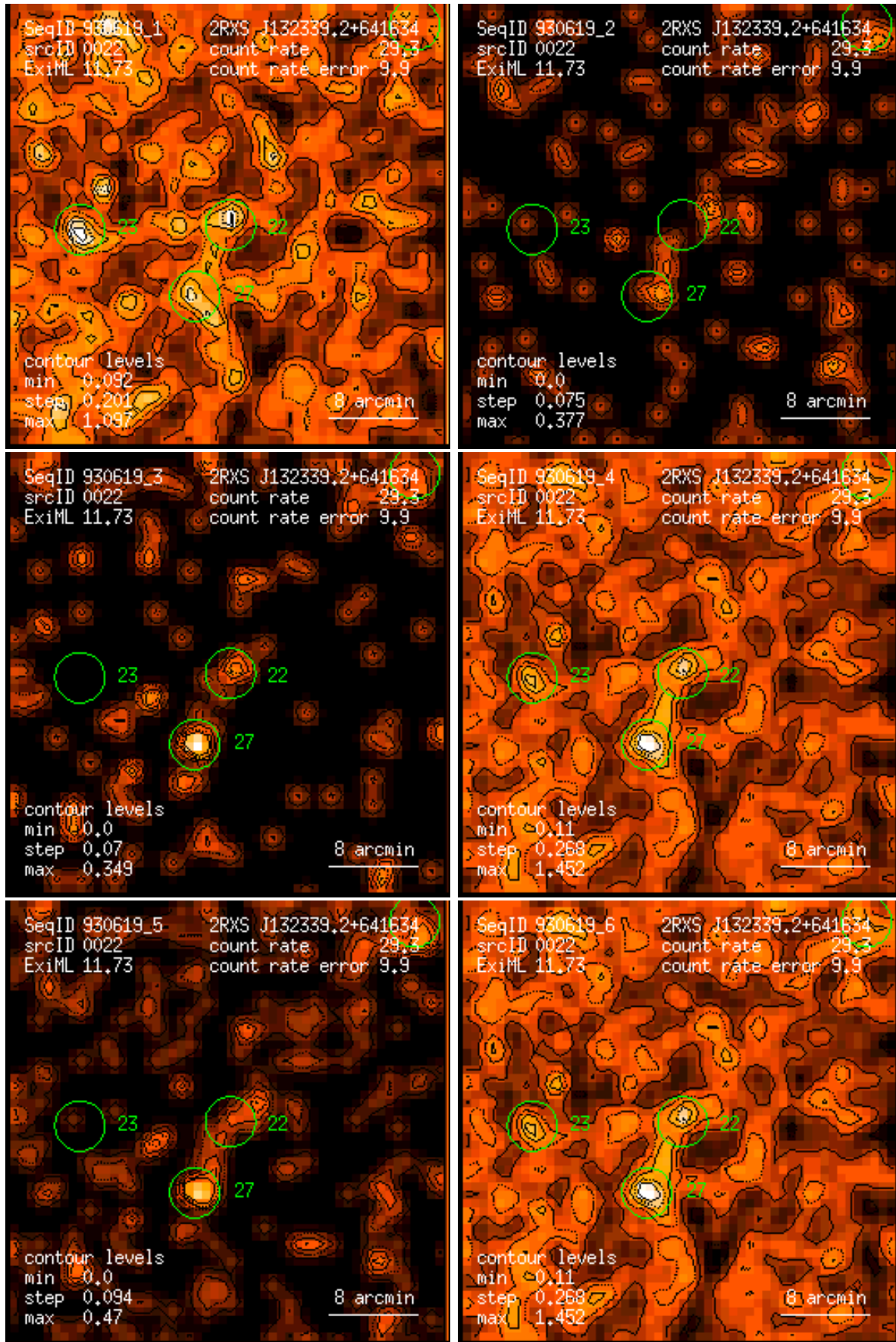
Figure 22: RASS 930619: detection 0022: band rate images, Gaussian filter: (1) PSPC channels 11 – 41, (2) 52 – 90, (3) 91 – 201, (4) 11 – 235, (5) 52 – 201, (6) 11 – 201. Broad band rates in counts/ks. Band rate contour levels in counts/ks/arcmin 2 .
