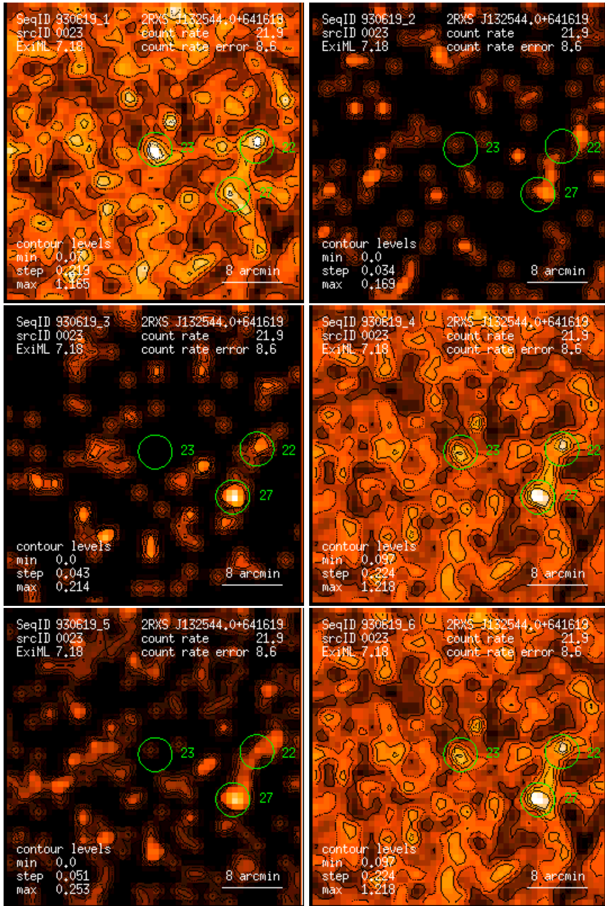
Figure 23: RASS 930619: detection 0023: band rate images, Gaussian filter: (1) PSPC channels 11 – 41, (2) 52 – 90, (3) 91 – 201, (4) 11 – 235, (5) 52 – 201, (6) 11 – 201. Broad band rates in counts/ks. Band rate contour levels in counts/ks/arcmin 2 .
