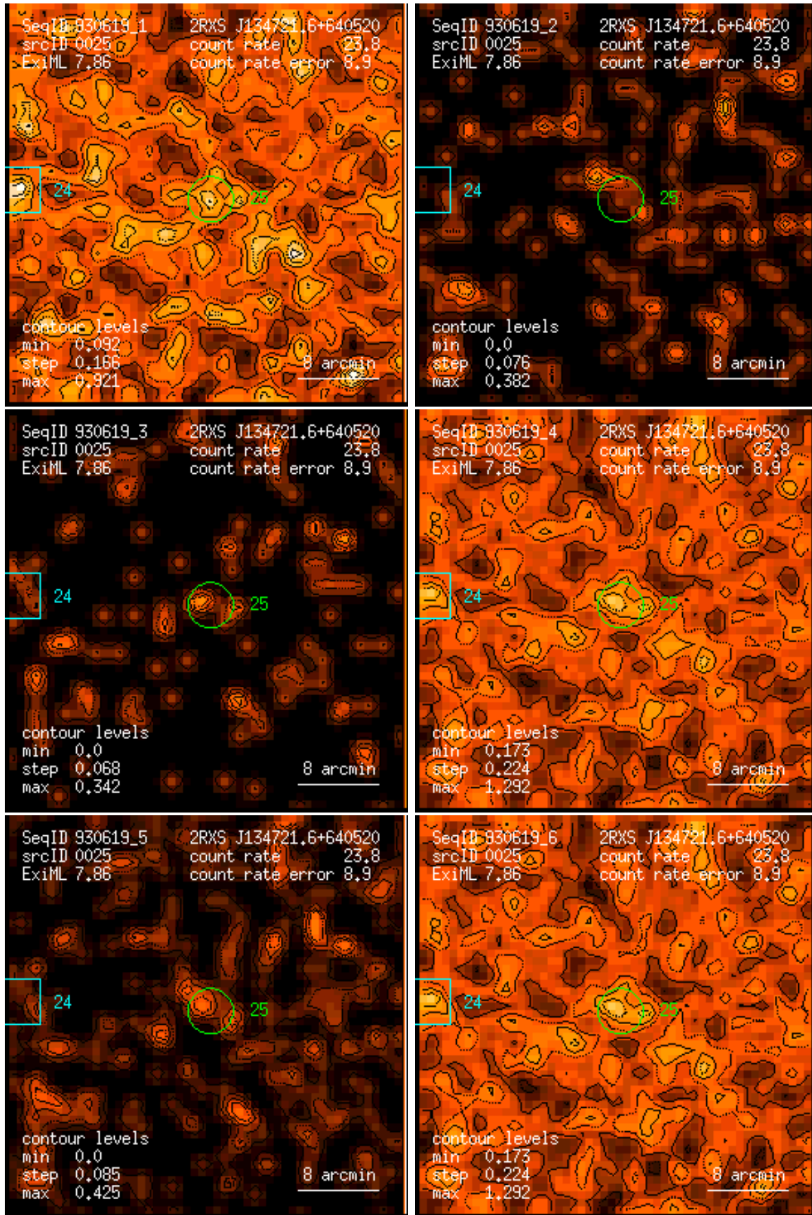
Figure 25: RASS 930619: detection 0025: band rate images, Gaussian filter: (1) PSPC channels 11 – 41, (2) 52 – 90, (3) 91 – 201, (4) 11 – 235, (5) 52 – 201, (6) 11 – 201. Broad band rates in counts/ks. Band rate contour levels in counts/ks/arcmin 2 .
