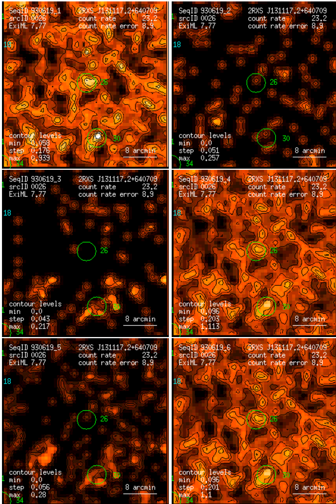
Figure 26: RASS 930619: detection 0026: band rate images, Gaussian filter: (1) PSPC channels 11 – 41, (2) 52 – 90, (3) 91 – 201, (4) 11 – 235, (5) 52 – 201, (6) 11 – 201. Broad band rates in counts/ks. Band rate contour levels in counts/ks/arcmin 2 .
