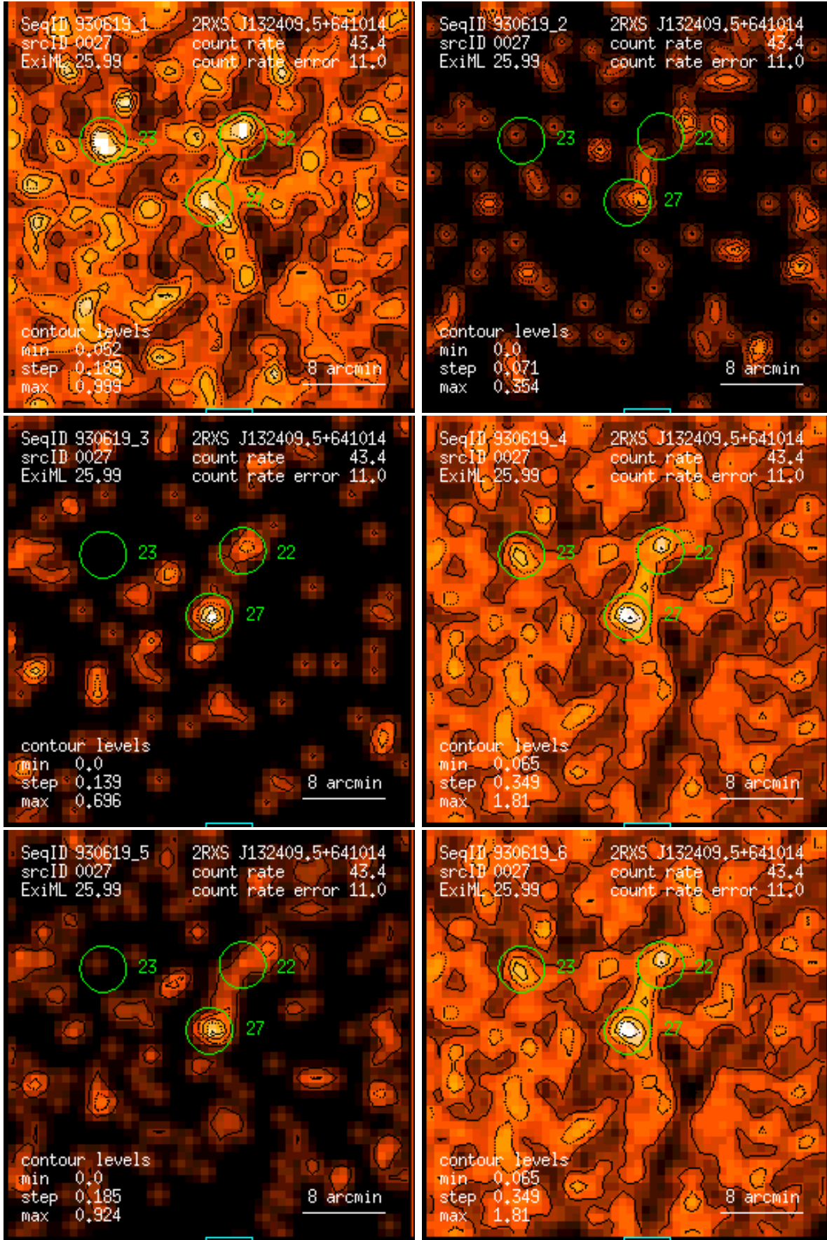
Figure 27: RASS 930619: detection 0027: band rate images, Gaussian filter: (1) PSPC channels 11 – 41, (2) 52 – 90, (3) 91 – 201, (4) 11 – 235, (5) 52 – 201, (6) 11 – 201. Broad band rates in counts/ks. Band rate contour levels in counts/ks/arcmin 2 .
