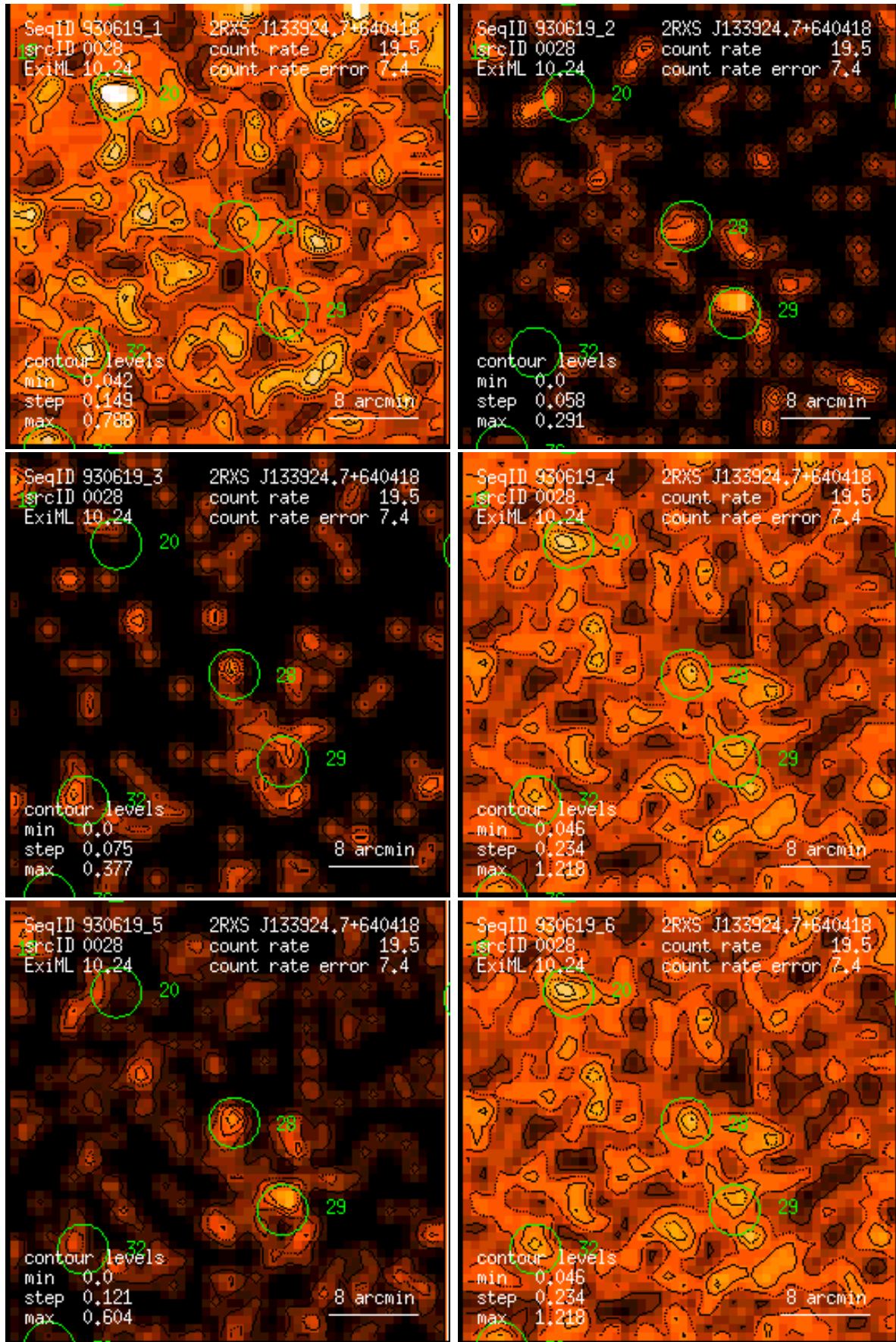
Figure 28: RASS 930619: detection 0028: band rate images, Gaussian filter: (1) PSPC channels 11 – 41, (2) 52 – 90, (3) 91 – 201, (4) 11 – 235, (5) 52 – 201, (6) 11 – 201. Broad band rates in counts/ks. Band rate contour levels in counts/ks/arcmin 2 .
