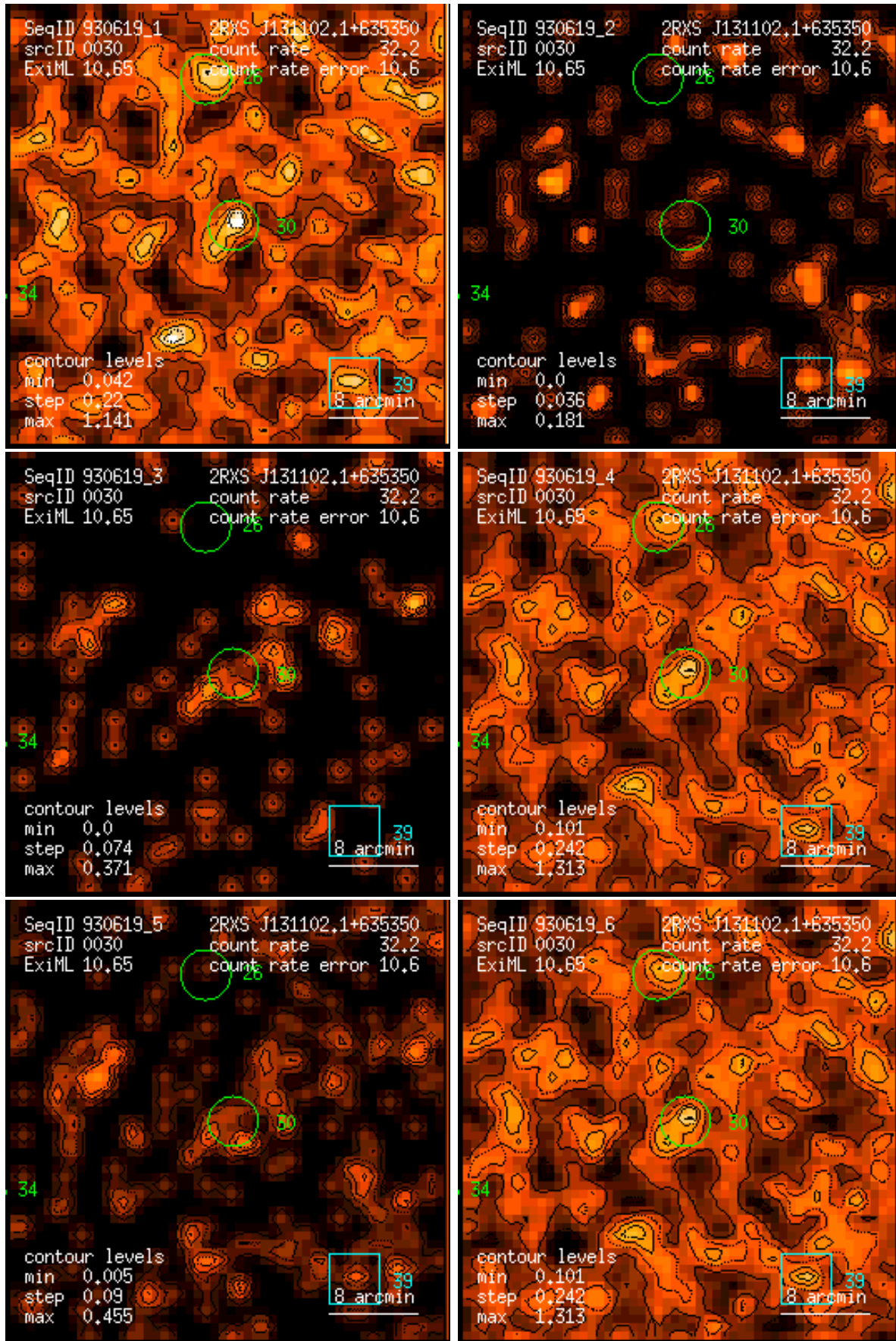
Figure 30: RASS 930619: detection 0030: band rate images, Gaussian filter: (1) PSPC channels 11 – 41, (2) 52 – 90, (3) 91 – 201, (4) 11 – 235, (5) 52 – 201, (6) 11 – 201. Broad band rates in counts/ks. Band rate contour levels in counts/ks/arcmin 2 .
