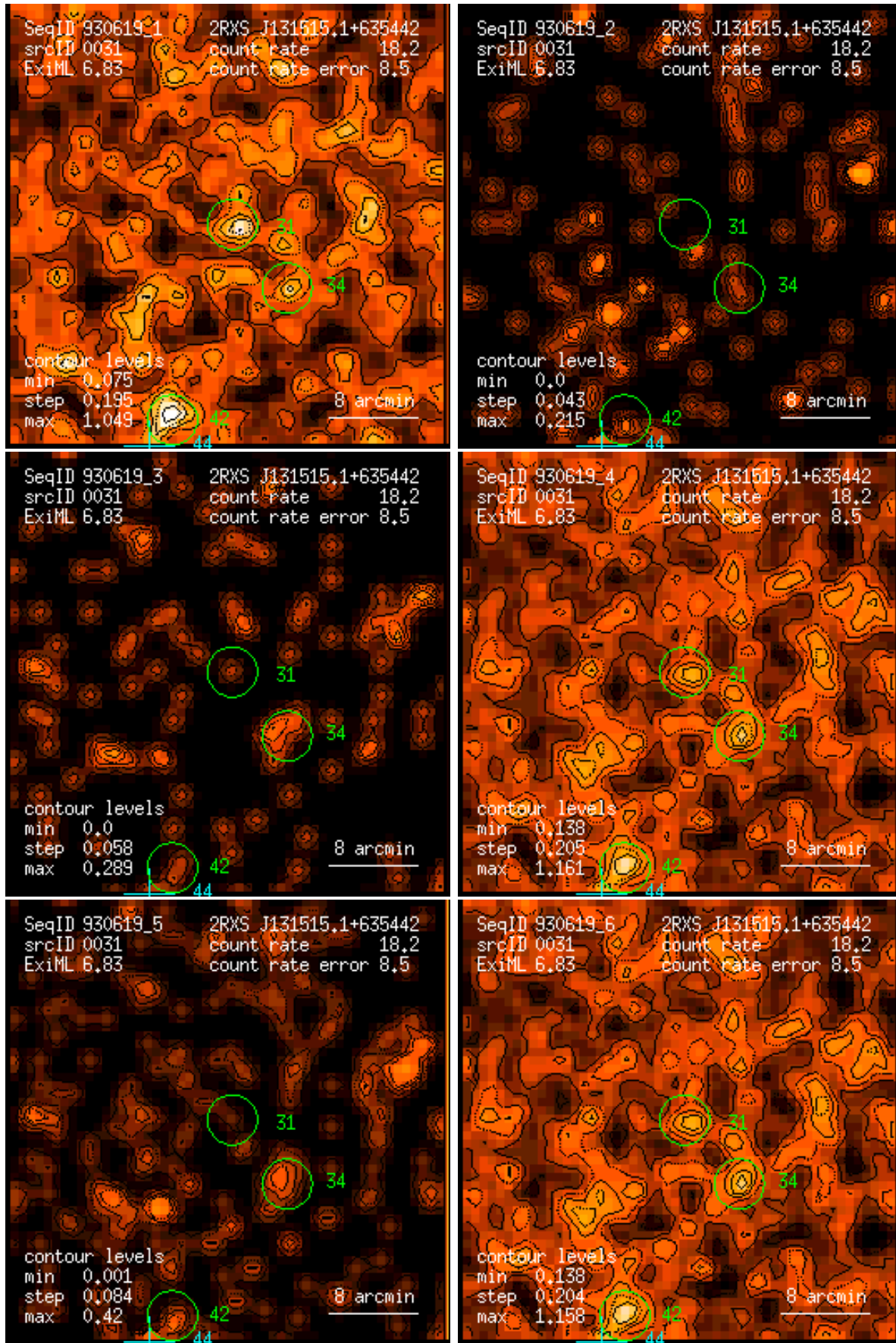
Figure 31: RASS 930619: detection 0031: band rate images, Gaussian filter: (1) PSPC channels 11 – 41, (2) 52 – 90, (3) 91 – 201, (4) 11 – 235, (5) 52 – 201, (6) 11 – 201. Broad band rates in counts/ks. Band rate contour levels in counts/ks/arcmin 2 .
