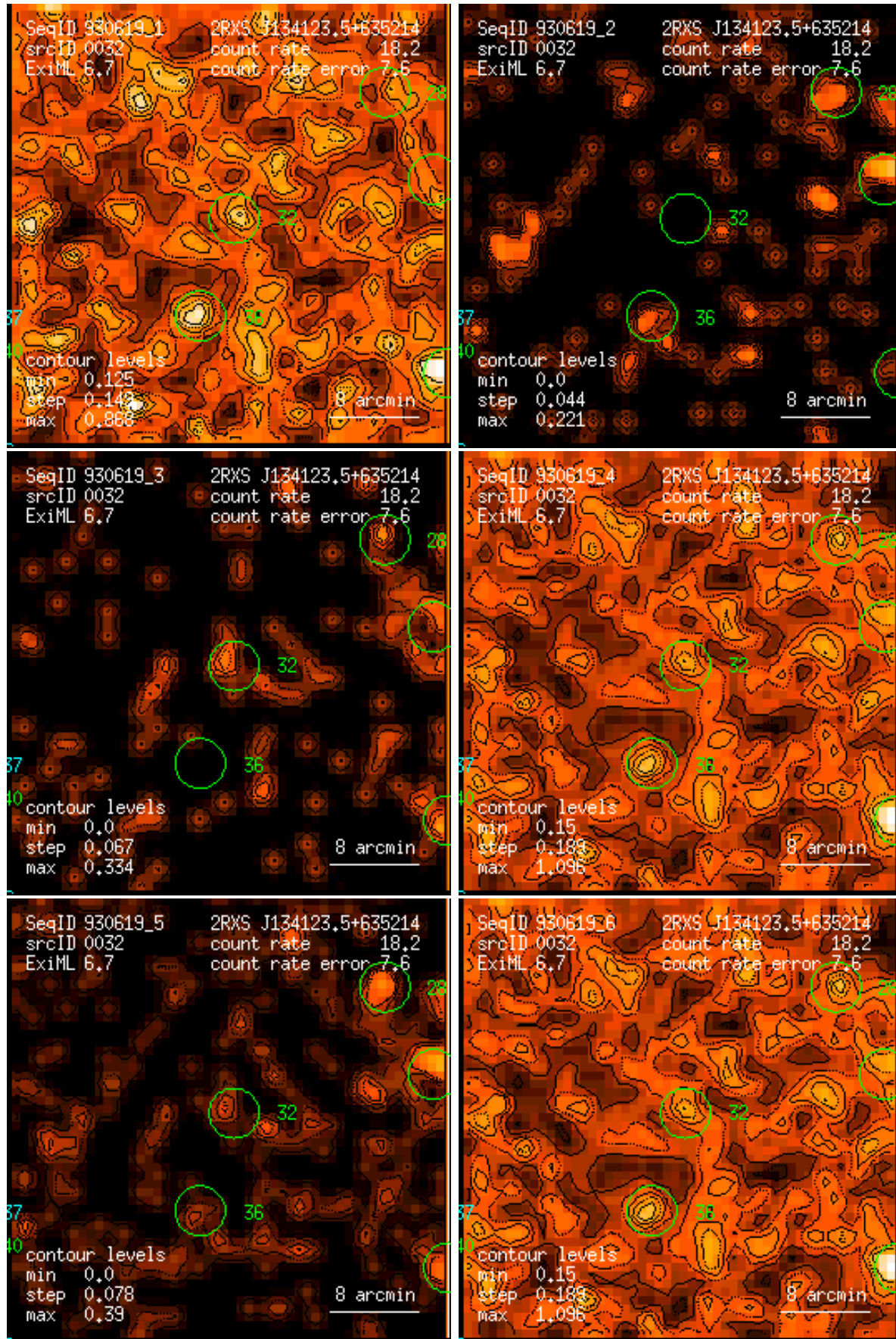
Figure 32: RASS 930619: detection 0032: band rate images, Gaussian filter: (1) PSPC channels 11 – 41, (2) 52 – 90, (3) 91 – 201, (4) 11 – 235, (5) 52 – 201, (6) 11 – 201. Broad band rates in counts/ks. Band rate contour levels in counts/ks/arcmin 2 .
