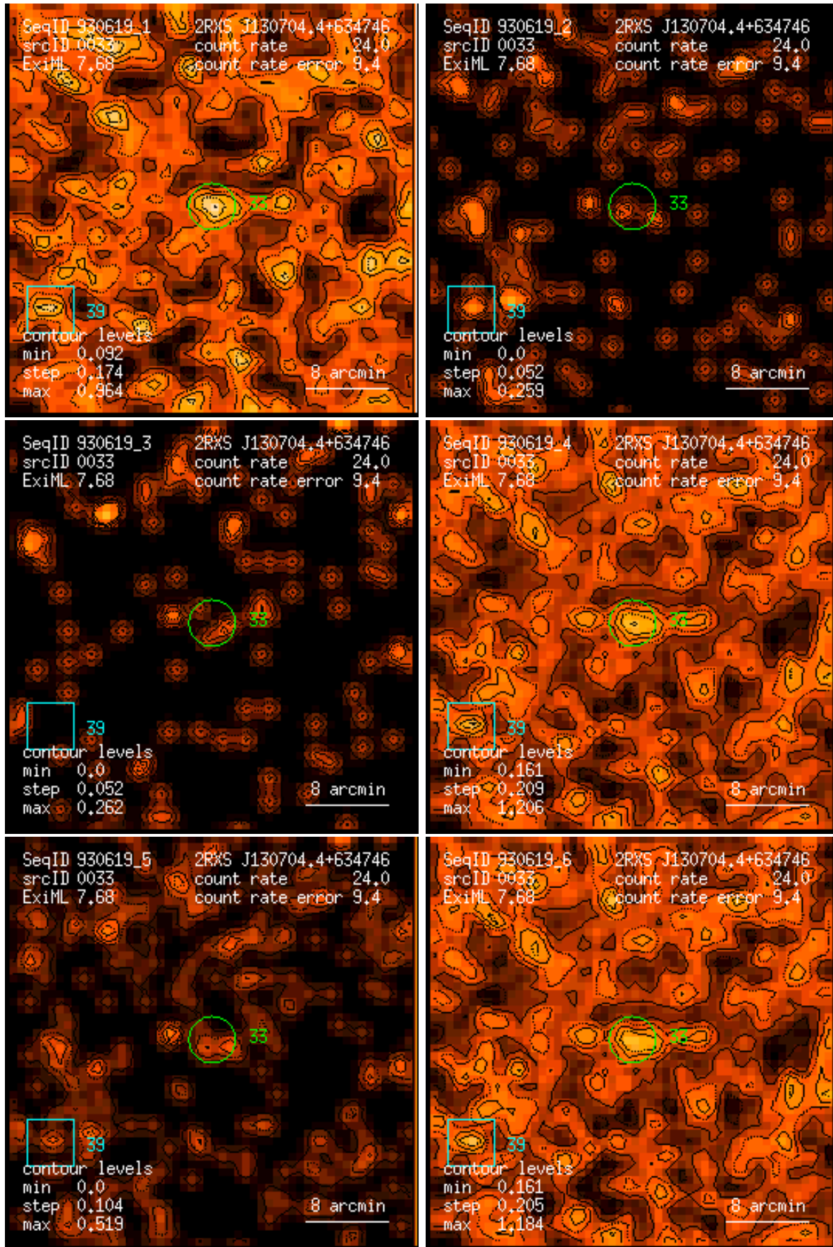
Figure 33: RASS 930619: detection 0033: band rate images, Gaussian filter: (1) PSPC channels 11 – 41, (2) 52 – 90, (3) 91 – 201, (4) 11 – 235, (5) 52 – 201, (6) 11 – 201. Broad band rates in counts/ks. Band rate contour levels in counts/ks/arcmin 2 .
