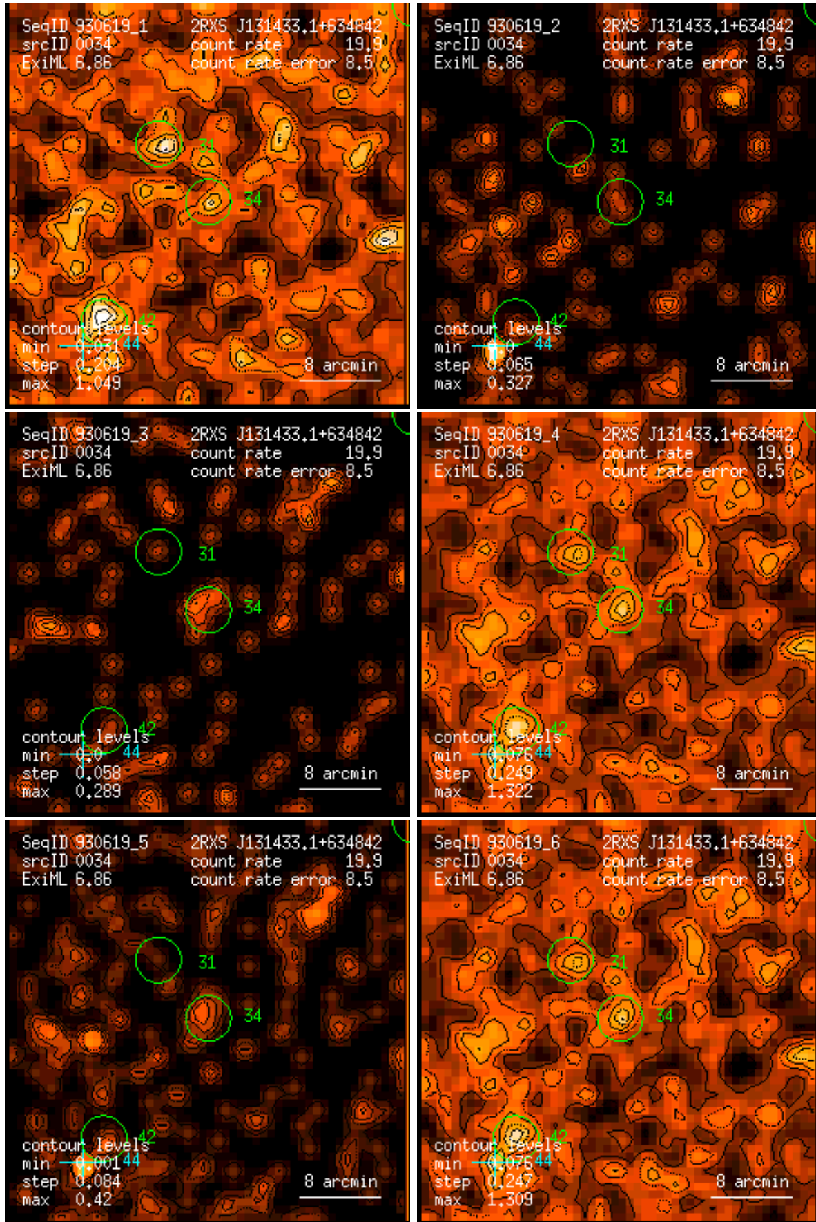
Figure 34: RASS 930619: detection 0034: band rate images, Gaussian filter: (1) PSPC channels 11 – 41, (2) 52 – 90, (3) 91 – 201, (4) 11 – 235, (5) 52 – 201, (6) 11 – 201. Broad band rates in counts/ks. Band rate contour levels in counts/ks/arcmin 2 .
