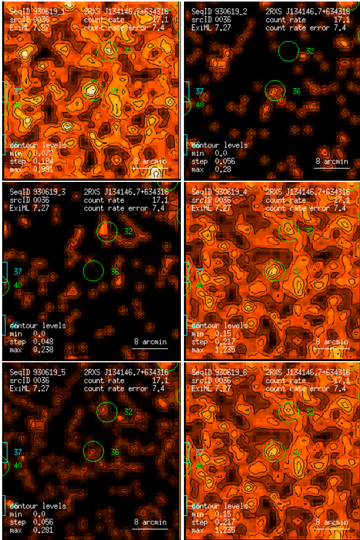
Figure 36: RASS 930619: detection 0036: band rate images, Gaussian filter: (1) PSPC channels 11 – 41, (2) 52 – 90, (3) 91 – 201, (4) 11 – 235, (5) 52 – 201, (6) 11 – 201. Broad band rates in counts/ks. Band rate contour levels in counts/ks/arcmin 2 .
