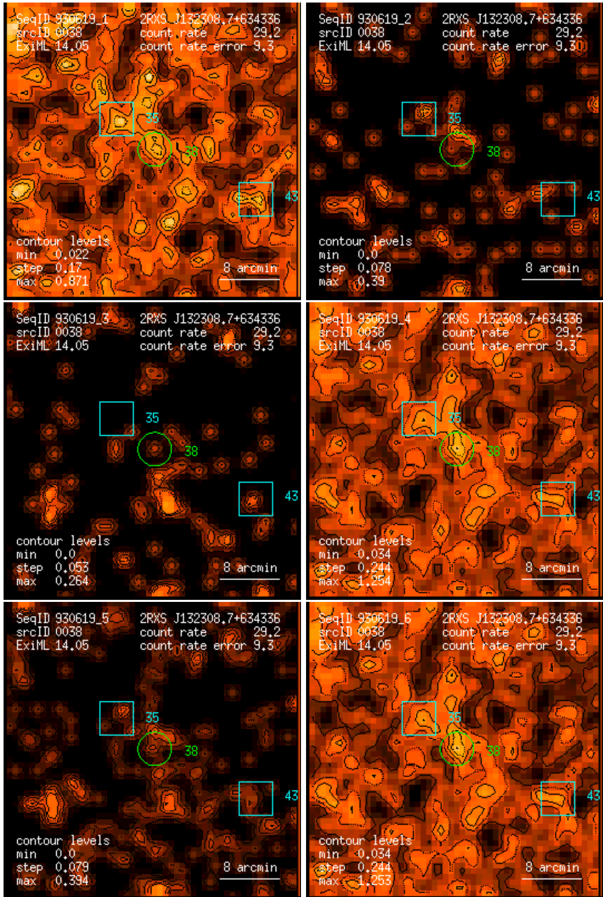
Figure 38: RASS 930619: detection 0038: band rate images, Gaussian filter: (1) PSPC channels 11 – 41, (2) 52 – 90, (3) 91 – 201, (4) 11 – 235, (5) 52 – 201, (6) 11 – 201. Broad band rates in counts/ks. Band rate contour levels in counts/ks/arcmin 2 .
