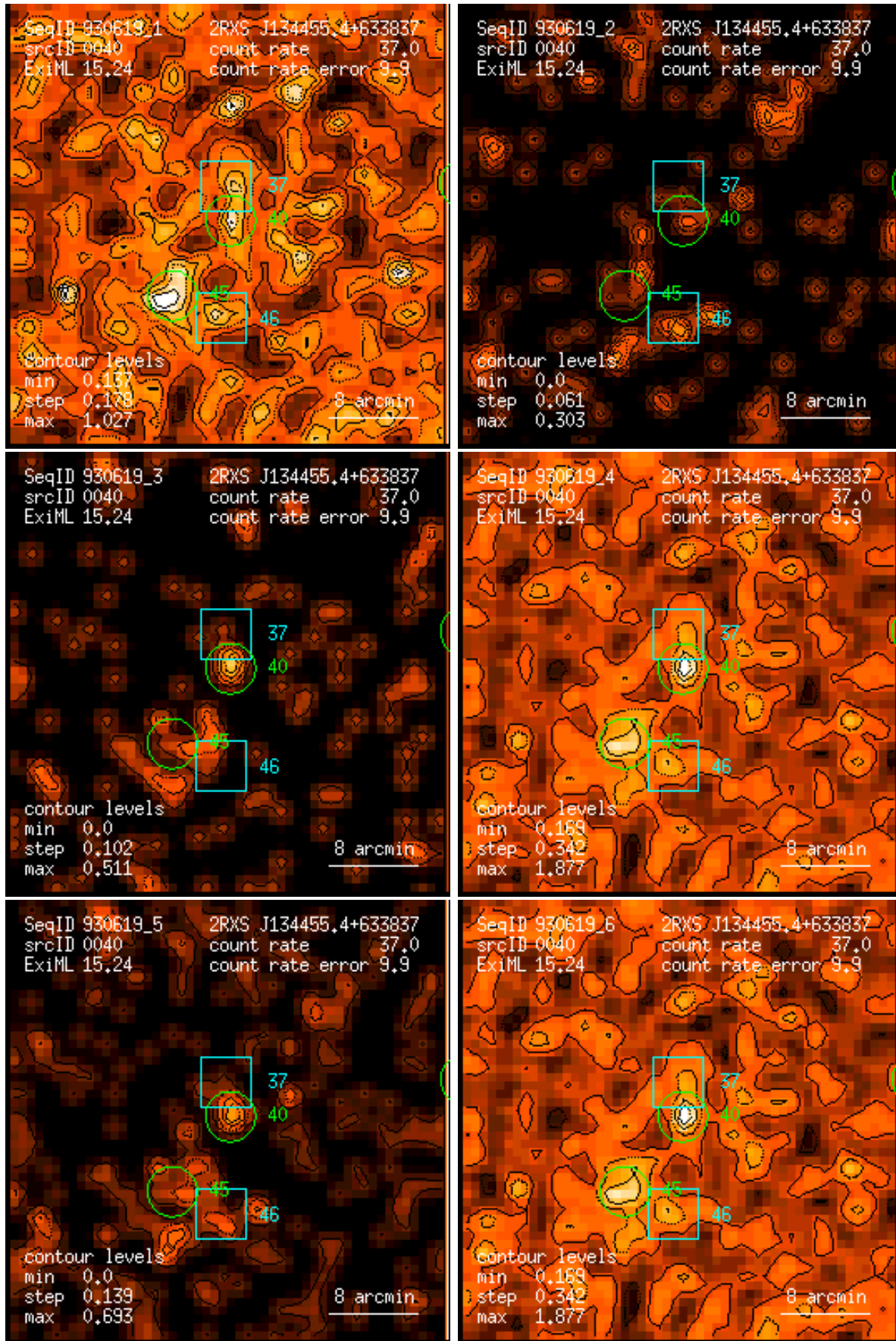
Figure 40: RASS 930619: detection 0040: band rate images, Gaussian filter: (1) PSPC channels 11 – 41, (2) 52 – 90, (3) 91 – 201, (4) 11 – 235, (5) 52 – 201, (6) 11 – 201. Broad band rates in counts/ks. Band rate contour levels in counts/ks/arcmin 2 .
