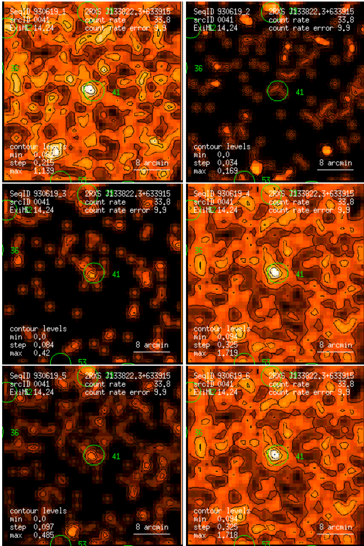
Figure 41: RASS 930619: detection 0041: band rate images, Gaussian filter: (1) PSPC channels 11 – 41, (2) 52 – 90, (3) 91 – 201, (4) 11 – 235, (5) 52 – 201, (6) 11 – 201. Broad band rates in counts/ks. Band rate contour levels in counts/ks/arcmin 2 .
