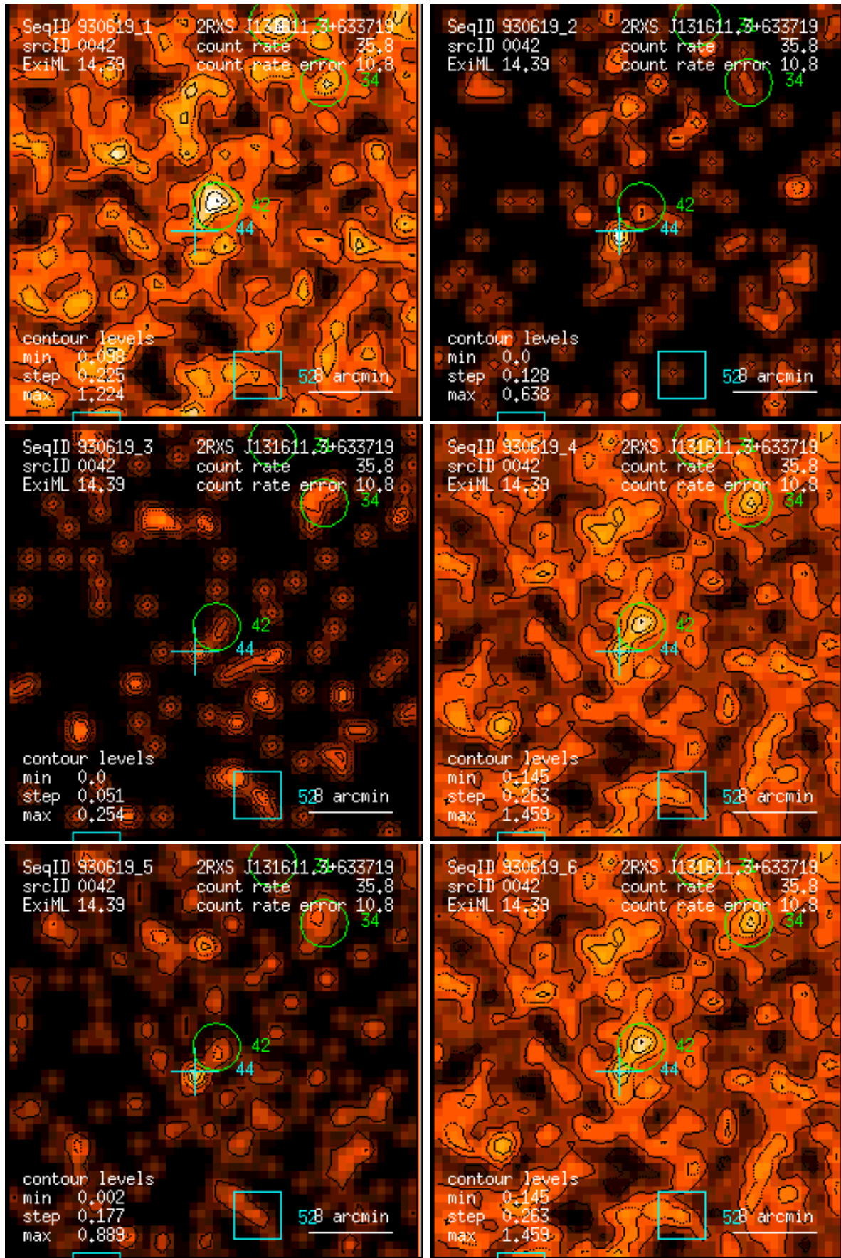
Figure 42: RASS 930619: detection 0042: band rate images, Gaussian filter: (1) PSPC channels 11 – 41, (2) 52 – 90, (3) 91 – 201, (4) 11 – 235, (5) 52 – 201, (6) 11 – 201. Broad band rates in counts/ks. Band rate contour levels in counts/ks/arcmin 2 .
