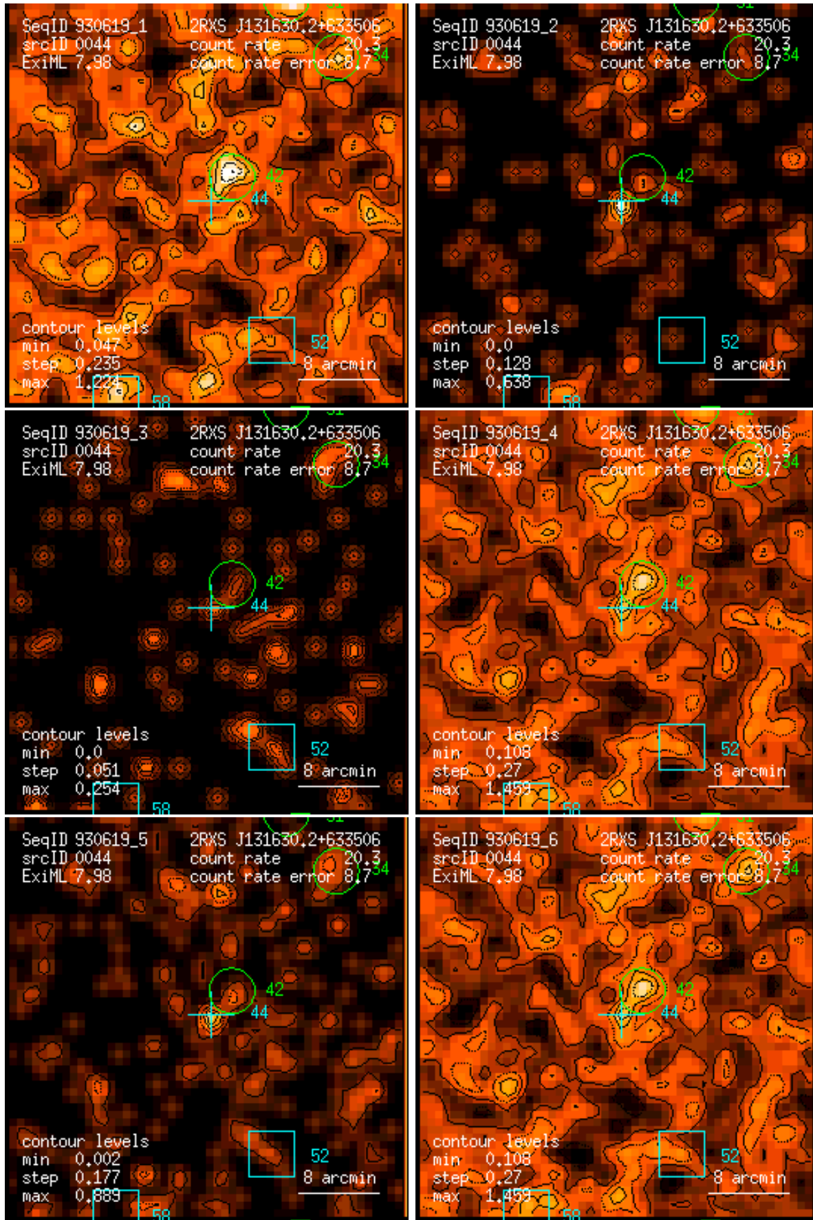
Figure 44: RASS 930619: detection 0044: band rate images, Gaussian filter: (1) PSPC channels 11 – 41, (2) 52 – 90, (3) 91 – 201, (4) 11 – 235, (5) 52 – 201, (6) 11 – 201. Broad band rates in counts/ks. Band rate contour levels in counts/ks/arcmin 2 .
