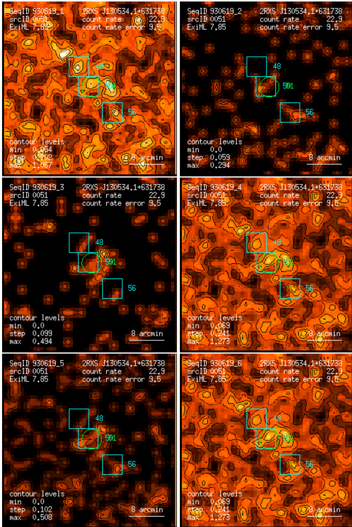
Figure 51: RASS 930619: detection 0051: band rate images, Gaussian filter: (1) PSPC channels 11 – 41, (2) 52 – 90, (3) 91 – 201, (4) 11 – 235, (5) 52 – 201, (6) 11 – 201. Broad band rates in counts/ks. Band rate contour levels in counts/ks/arcmin 2 .
