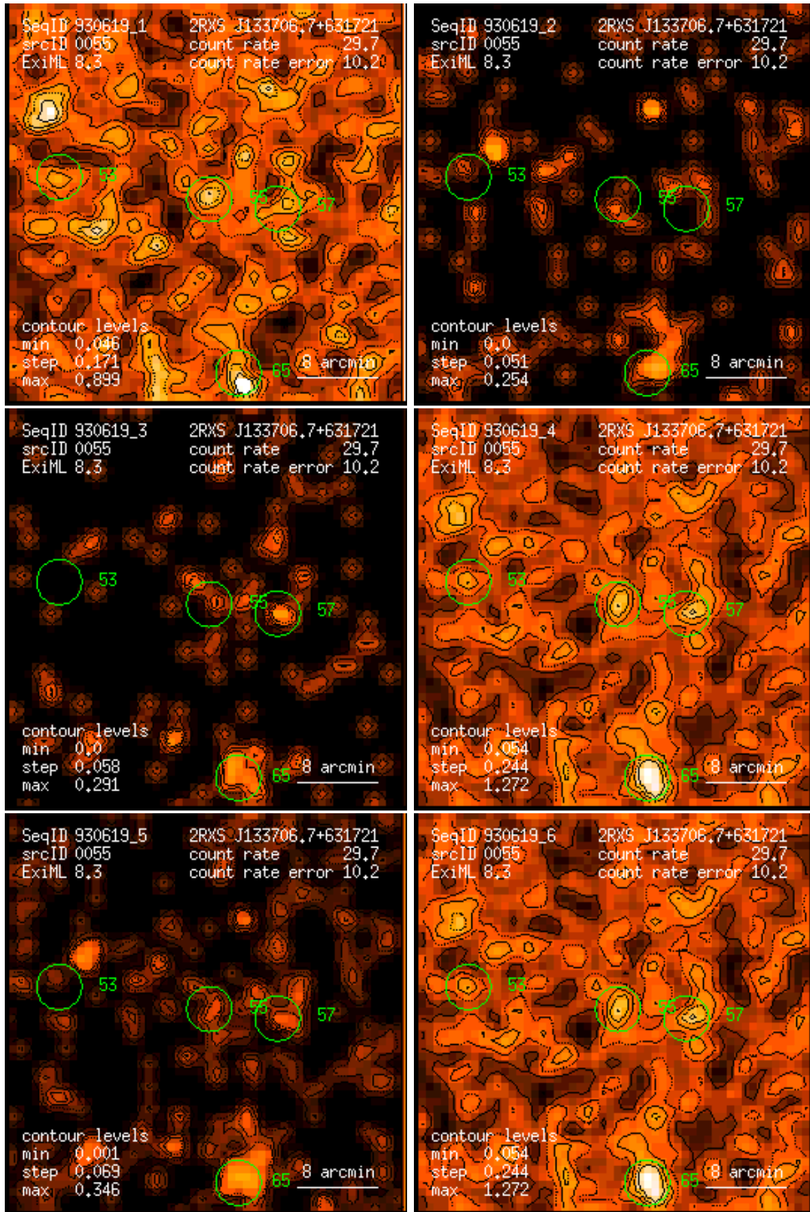
Figure 55: RASS 930619: detection 0055: band rate images, Gaussian filter: (1) PSPC channels 11 – 41, (2) 52 – 90, (3) 91 – 201, (4) 11 – 235, (5) 52 – 201, (6) 11 – 201. Broad band rates in counts/ks. Band rate contour levels in counts/ks/arcmin 2 .
