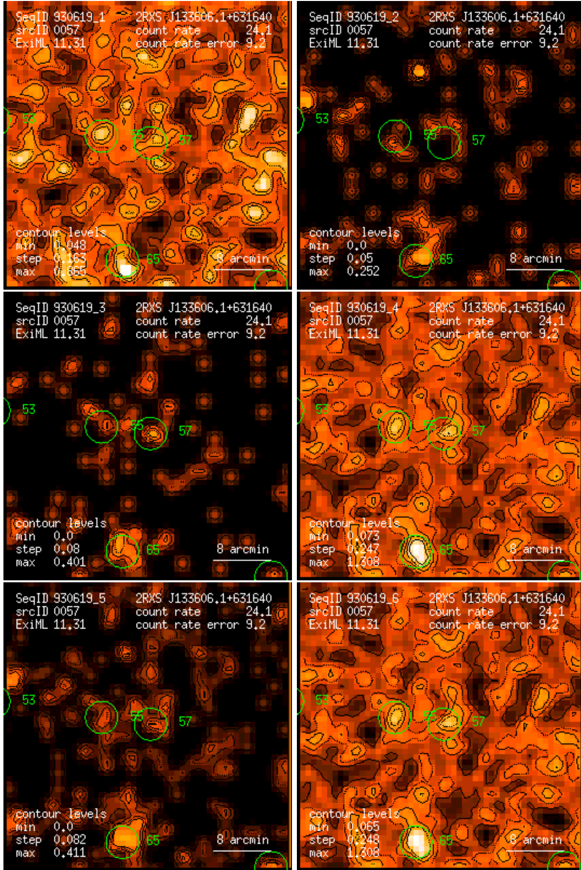
Figure 57: RASS 930619: detection 0057: band rate images, Gaussian filter: (1) PSPC channels 11 – 41, (2) 52 – 90, (3) 91 – 201, (4) 11 – 235, (5) 52 – 201, (6) 11 – 201. Broad band rates in counts/ks. Band rate contour levels in counts/ks/arcmin 2 .
