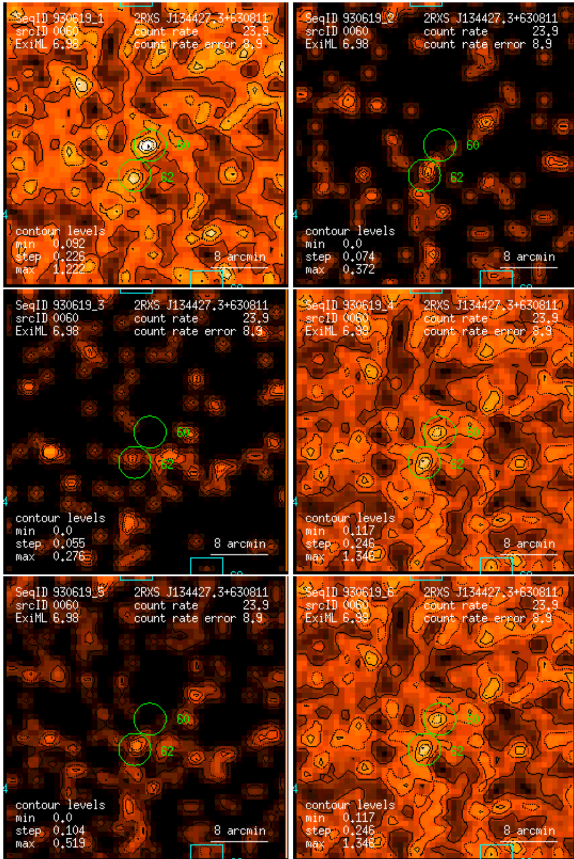
Figure 60: RASS 930619: detection 0060: band rate images, Gaussian filter: (1) PSPC channels 11 – 41, (2) 52 – 90, (3) 91 – 201, (4) 11 – 235, (5) 52 – 201, (6) 11 – 201. Broad band rates in counts/ks. Band rate contour levels in counts/ks/arcmin 2 .
