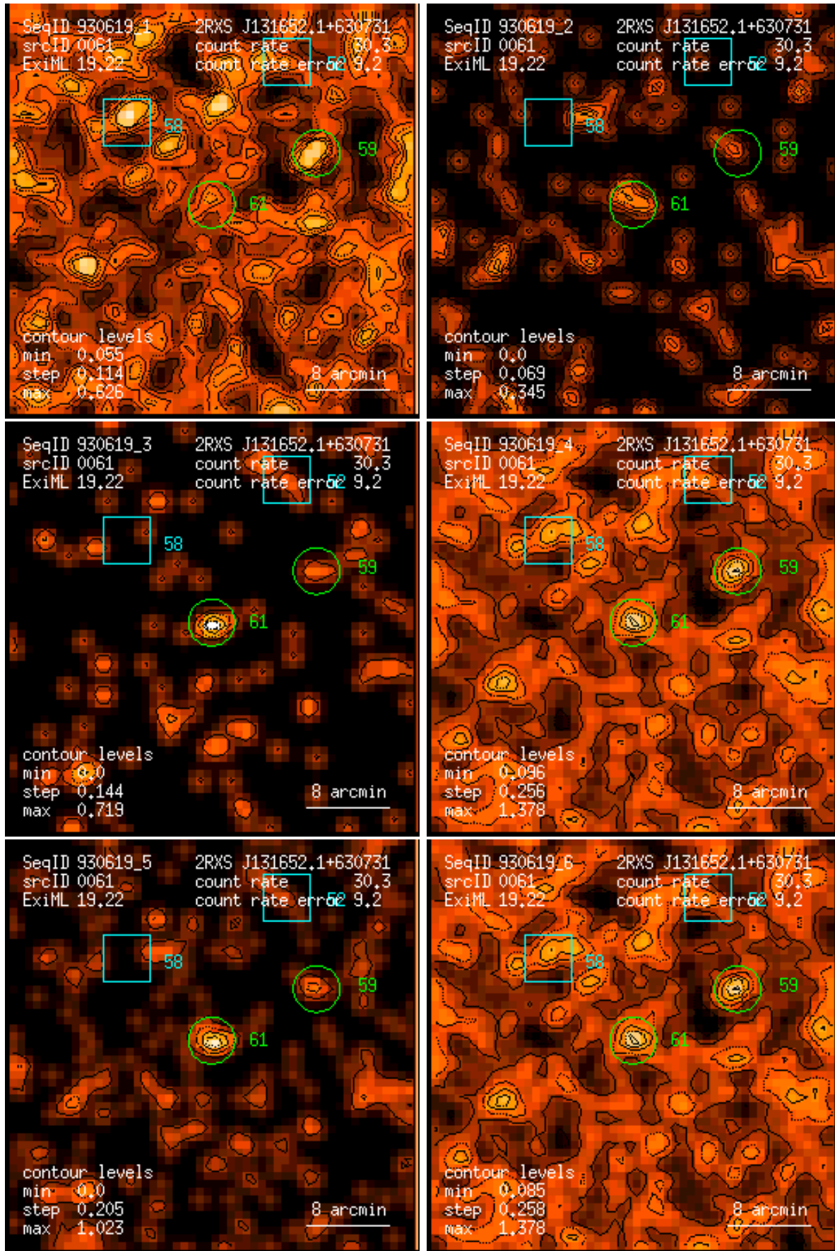
Figure 61: RASS 930619: detection 0061: band rate images, Gaussian filter: (1) PSPC channels 11 – 41, (2) 52 – 90, (3) 91 – 201, (4) 11 – 235, (5) 52 – 201, (6) 11 – 201. Broad band rates in counts/ks. Band rate contour levels in counts/ks/arcmin 2 .
