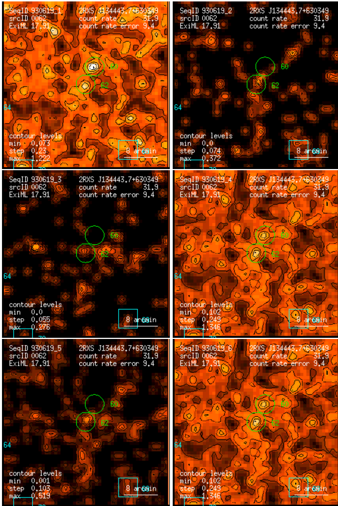
Figure 62: RASS 930619: detection 0062: band rate images, Gaussian filter: (1) PSPC channels 11 – 41, (2) 52 – 90, (3) 91 – 201, (4) 11 – 235, (5) 52 – 201, (6) 11 – 201. Broad band rates in counts/ks. Band rate contour levels in counts/ks/arcmin 2 .
