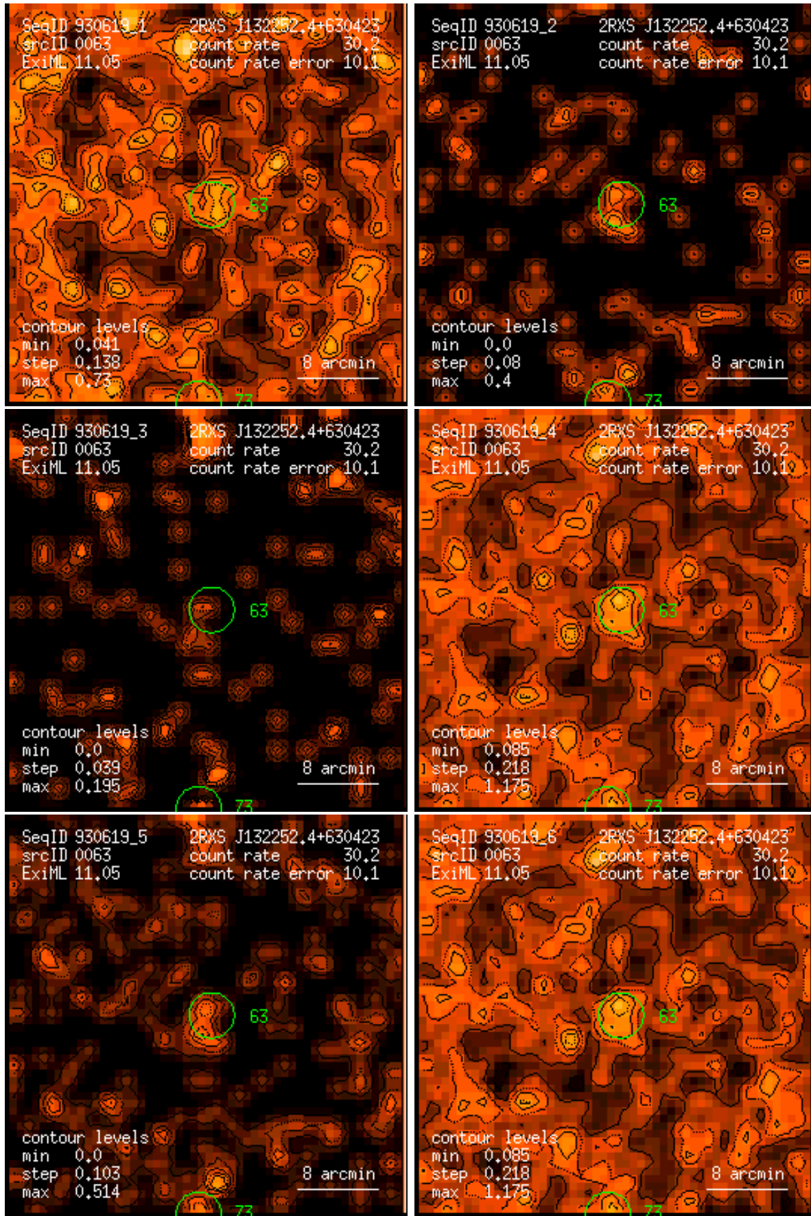
Figure 63: RASS 930619: detection 0063: band rate images, Gaussian filter: (1) PSPC channels 11 – 41, (2) 52 – 90, (3) 91 – 201, (4) 11 – 235, (5) 52 – 201, (6) 11 – 201. Broad band rates in counts/ks. Band rate contour levels in counts/ks/arcmin 2 .
