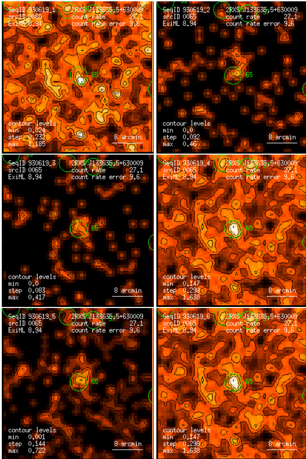
Figure 65: RASS 930619: detection 0065: band rate images, Gaussian filter: (1) PSPC channels 11 – 41, (2) 52 – 90, (3) 91 – 201, (4) 11 – 235, (5) 52 – 201, (6) 11 – 201. Broad band rates in counts/ks. Band rate contour levels in counts/ks/arcmin 2 .
