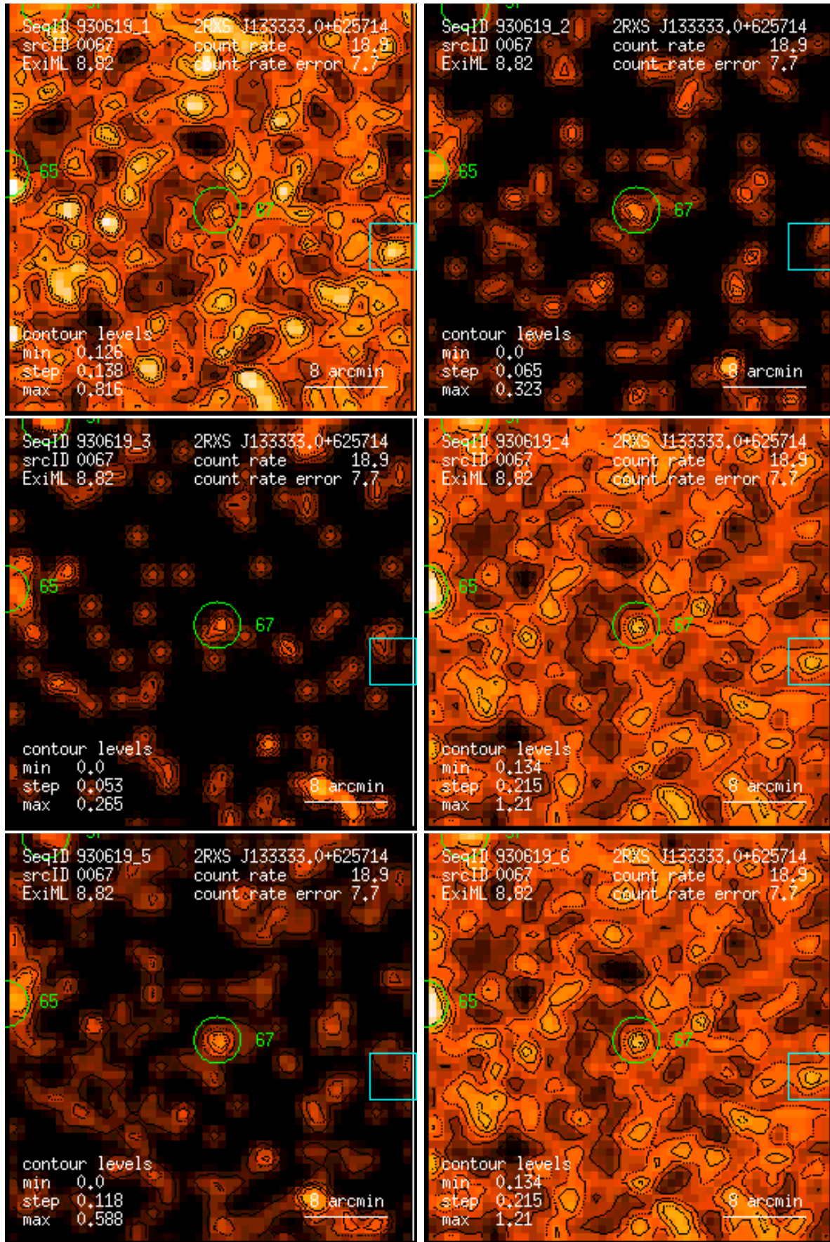
Figure 67: RASS 930619: detection 0067: band rate images, Gaussian filter: (1) PSPC channels 11 – 41, (2) 52 – 90, (3) 91 – 201, (4) 11 – 235, (5) 52 – 201, (6) 11 – 201. Broad band rates in counts/ks. Band rate contour levels in counts/ks/arcmin 2 .
