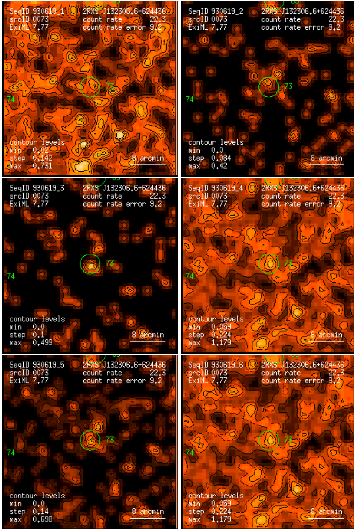
Figure 73: RASS 930619: detection 0073: band rate images, Gaussian filter: (1) PSPC channels 11 – 41, (2) 52 – 90, (3) 91 – 201, (4) 11 – 235, (5) 52 – 201, (6) 11 – 201. Broad band rates in counts/ks. Band rate contour levels in counts/ks/arcmin 2 .
