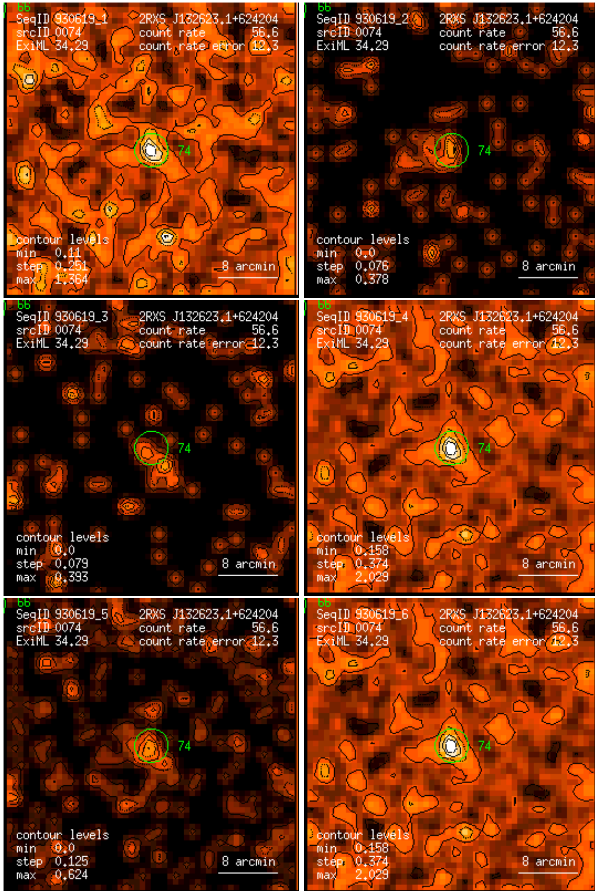
Figure 74: RASS 930619: detection 0074: band rate images, Gaussian filter: (1) PSPC channels 11 – 41, (2) 52 – 90, (3) 91 – 201, (4) 11 – 235, (5) 52 – 201, (6) 11 – 201. Broad band rates in counts/ks. Band rate contour levels in counts/ks/arcmin 2 .
