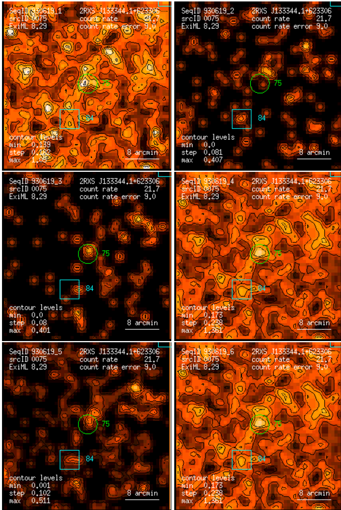
Figure 75: RASS 930619: detection 0075: band rate images, Gaussian filter: (1) PSPC channels 11 – 41, (2) 52 – 90, (3) 91 – 201, (4) 11 – 235, (5) 52 – 201, (6) 11 – 201. Broad band rates in counts/ks. Band rate contour levels in counts/ks/arcmin 2 .
