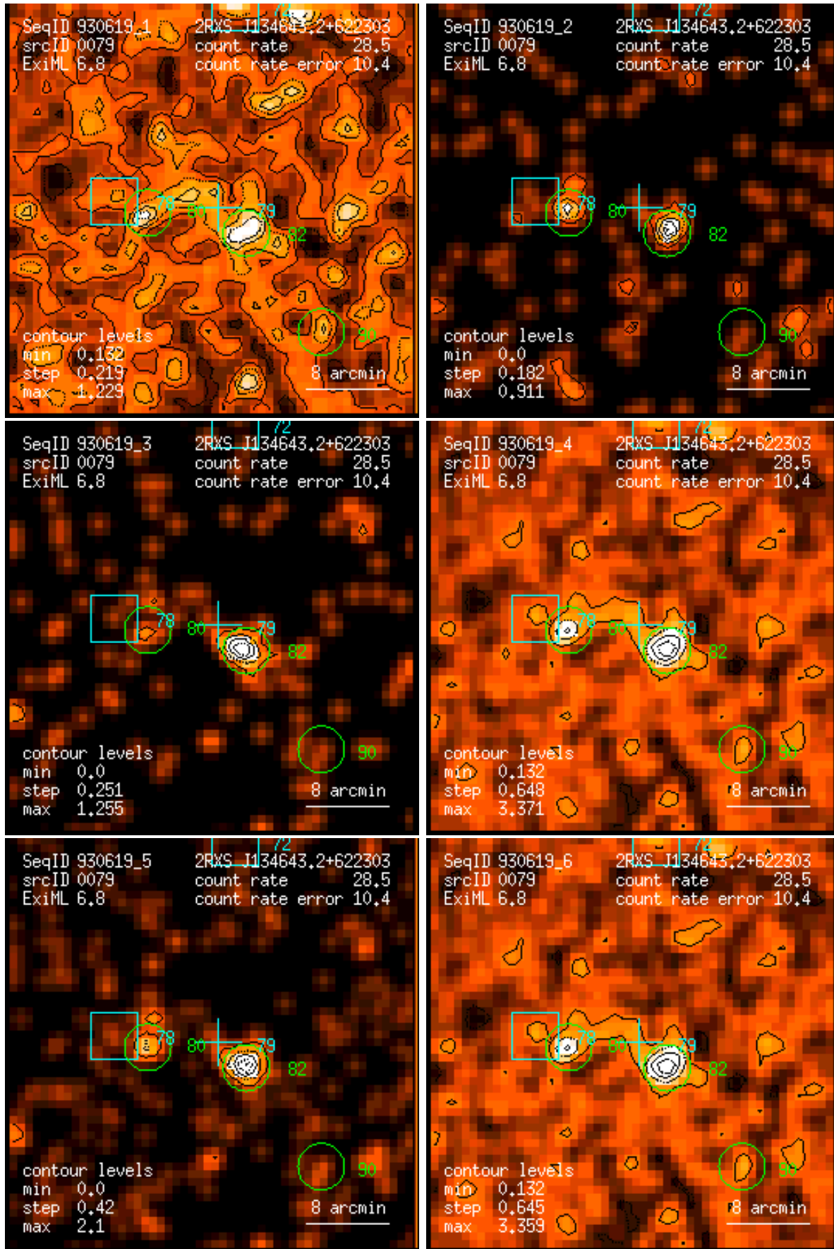
Figure 79: RASS 930619: detection 0079: band rate images, Gaussian filter: (1) PSPC channels 11 – 41, (2) 52 – 90, (3) 91 – 201, (4) 11 – 235, (5) 52 – 201, (6) 11 – 201. Broad band rates in counts/ks. Band rate contour levels in counts/ks/arcmin 2 .
