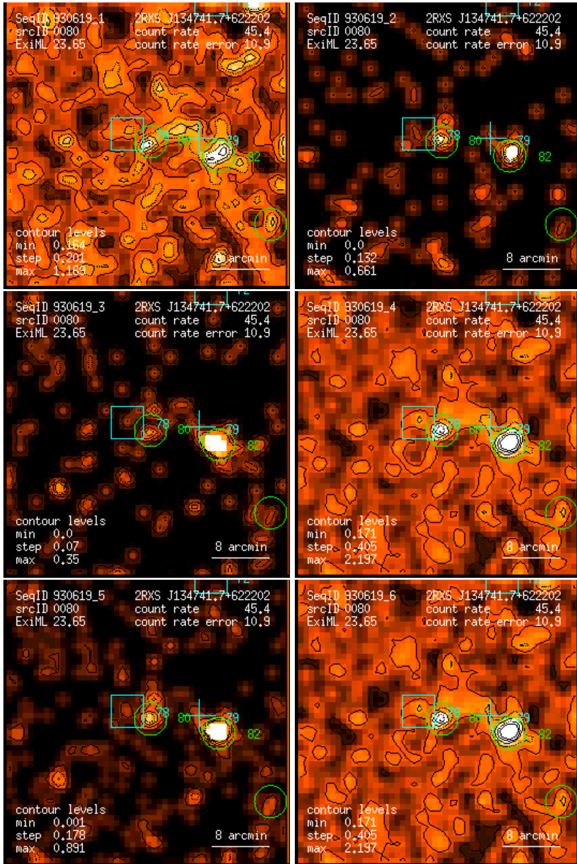
Figure 80: RASS 930619: detection 0080: band rate images, Gaussian filter: (1) PSPC channels 11 – 41, (2) 52 – 90, (3) 91 – 201, (4) 11 – 235, (5) 52 – 201, (6) 11 – 201. Broad band rates in counts/ks. Band rate contour levels in counts/ks/arcmin 2 .
