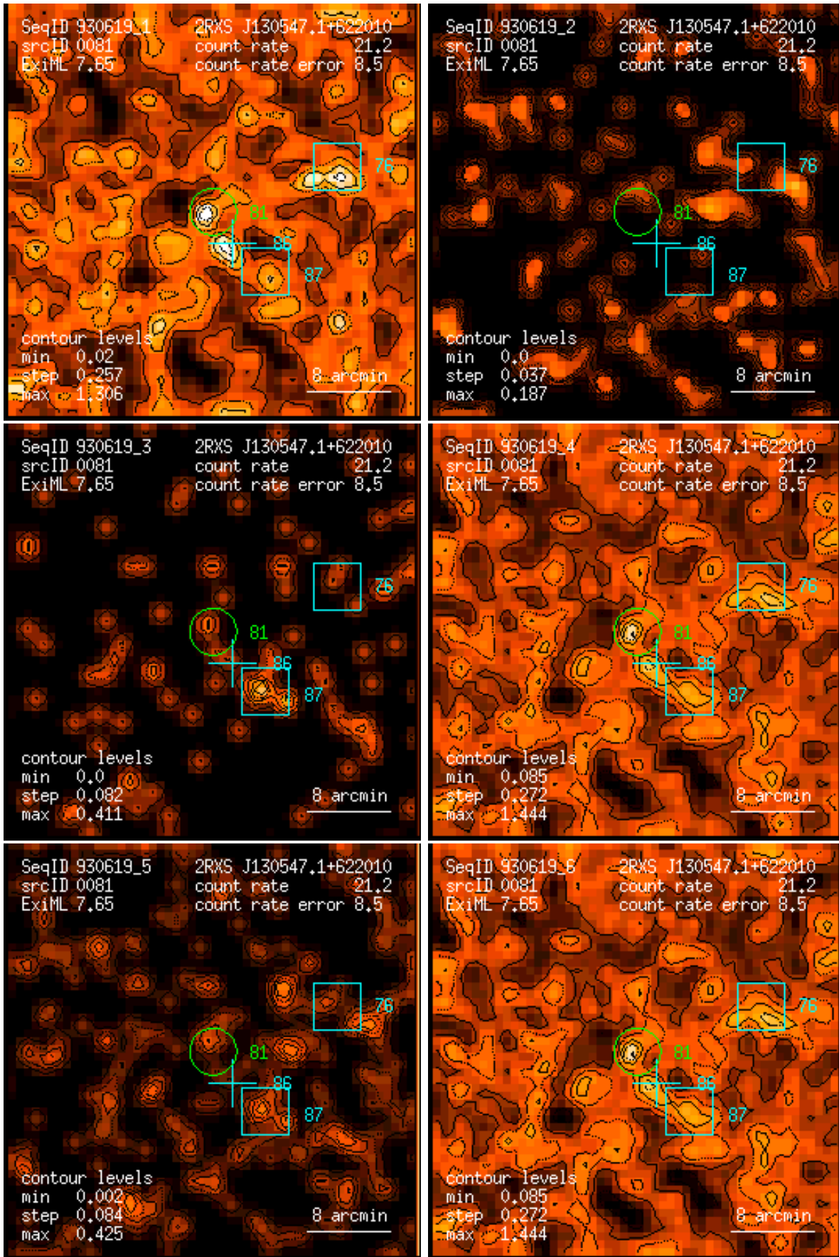
Figure 81: RASS 930619: detection 0081: band rate images, Gaussian filter: (1) PSPC channels 11 – 41, (2) 52 – 90, (3) 91 – 201, (4) 11 – 235, (5) 52 – 201, (6) 11 – 201. Broad band rates in counts/ks. Band rate contour levels in counts/ks/arcmin 2 .
