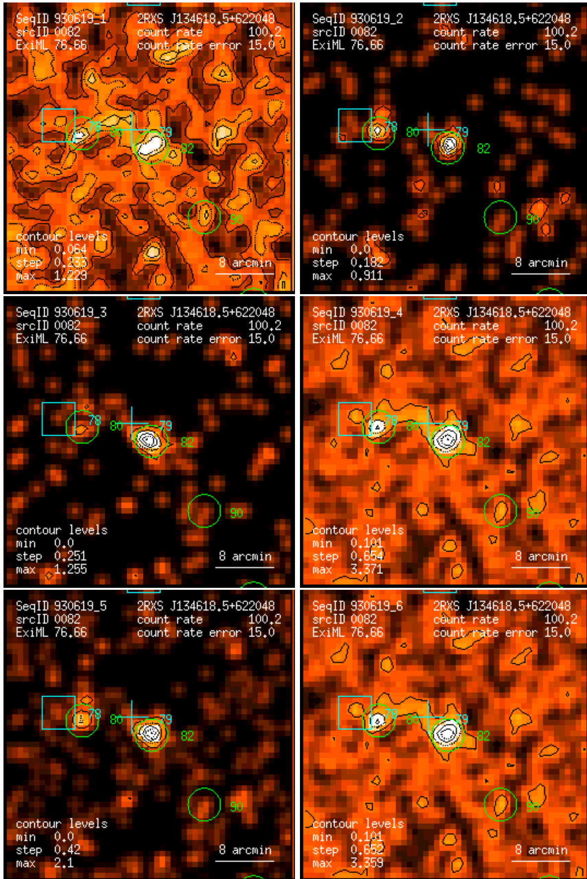
Figure 82: RASS 930619: detection 0082: band rate images, Gaussian filter: (1) PSPC channels 11 – 41, (2) 52 – 90, (3) 91 – 201, (4) 11 – 235, (5) 52 – 201, (6) 11 – 201. Broad band rates in counts/ks. Band rate contour levels in counts/ks/arcmin 2 .
