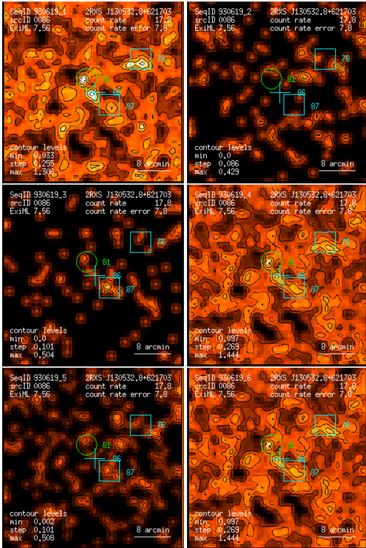
Figure 86: RASS 930619: detection 0086: band rate images, Gaussian filter: (1) PSPC channels 11 – 41, (2) 52 – 90, (3) 91 – 201, (4) 11 – 235, (5) 52 – 201, (6) 11 – 201. Broad band rates in counts/ks. Band rate contour levels in counts/ks/arcmin 2 .
