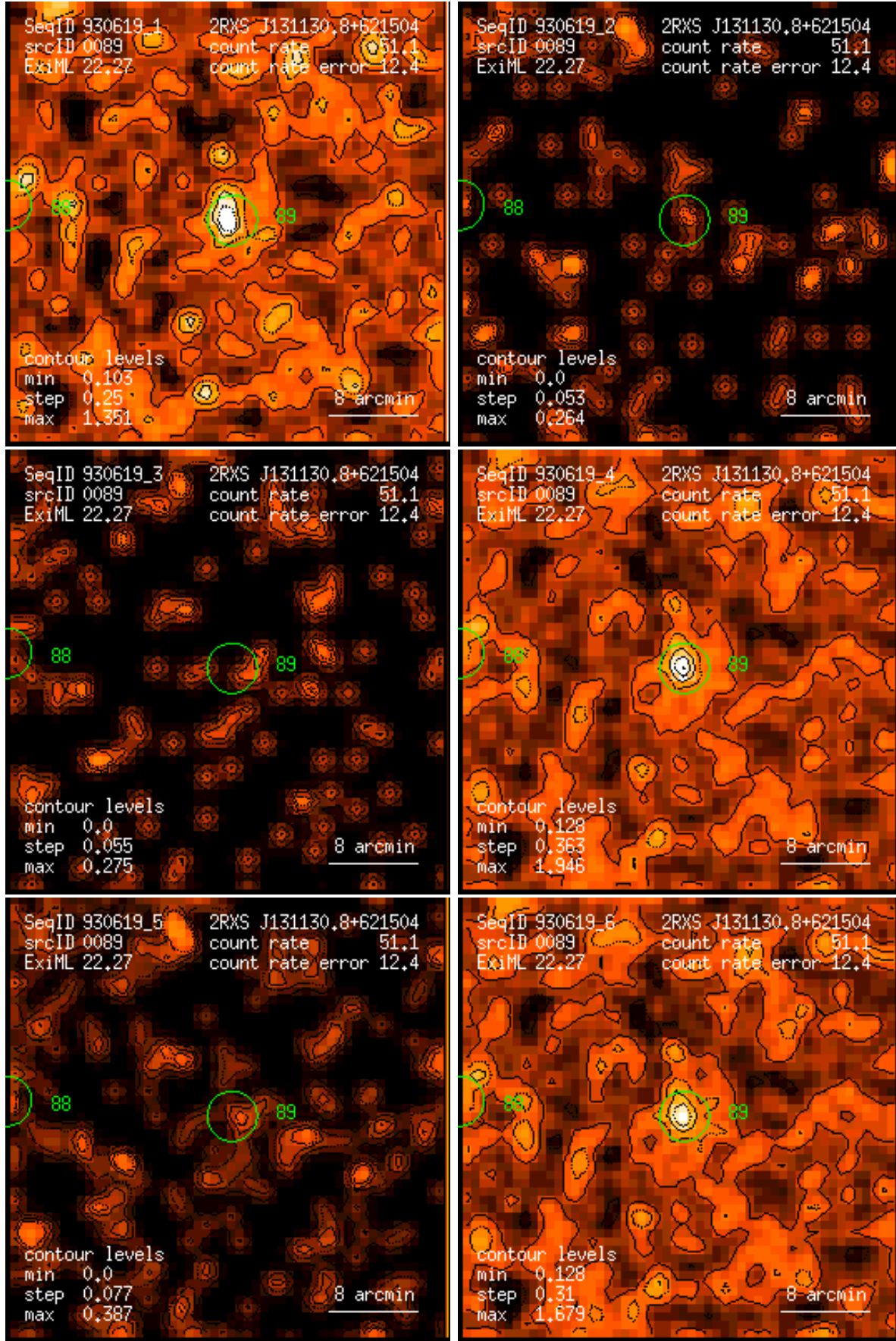
Figure 89: RASS 930619: detection 0089: band rate images, Gaussian filter: (1) PSPC channels 11 – 41, (2) 52 – 90, (3) 91 – 201, (4) 11 – 235, (5) 52 – 201, (6) 11 – 201. Broad band rates in counts/ks. Band rate contour levels in counts/ks/arcmin 2 .
