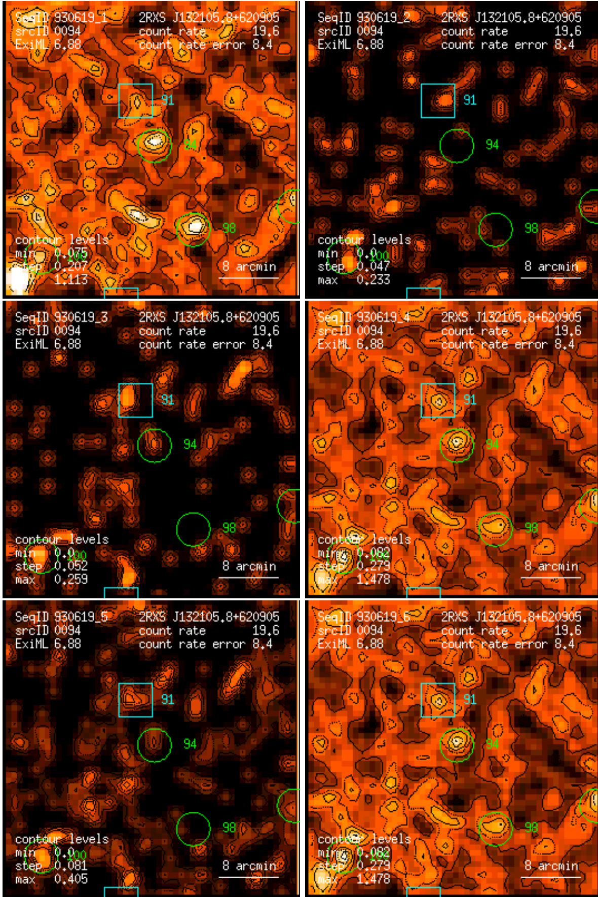
Figure 94: RASS 930619: detection 0094: band rate images, Gaussian filter: (1) PSPC channels 11 – 41, (2) 52 – 90, (3) 91 – 201, (4) 11 – 235, (5) 52 – 201, (6) 11 – 201. Broad band rates in counts/ks. Band rate contour levels in counts/ks/arcmin 2 .
