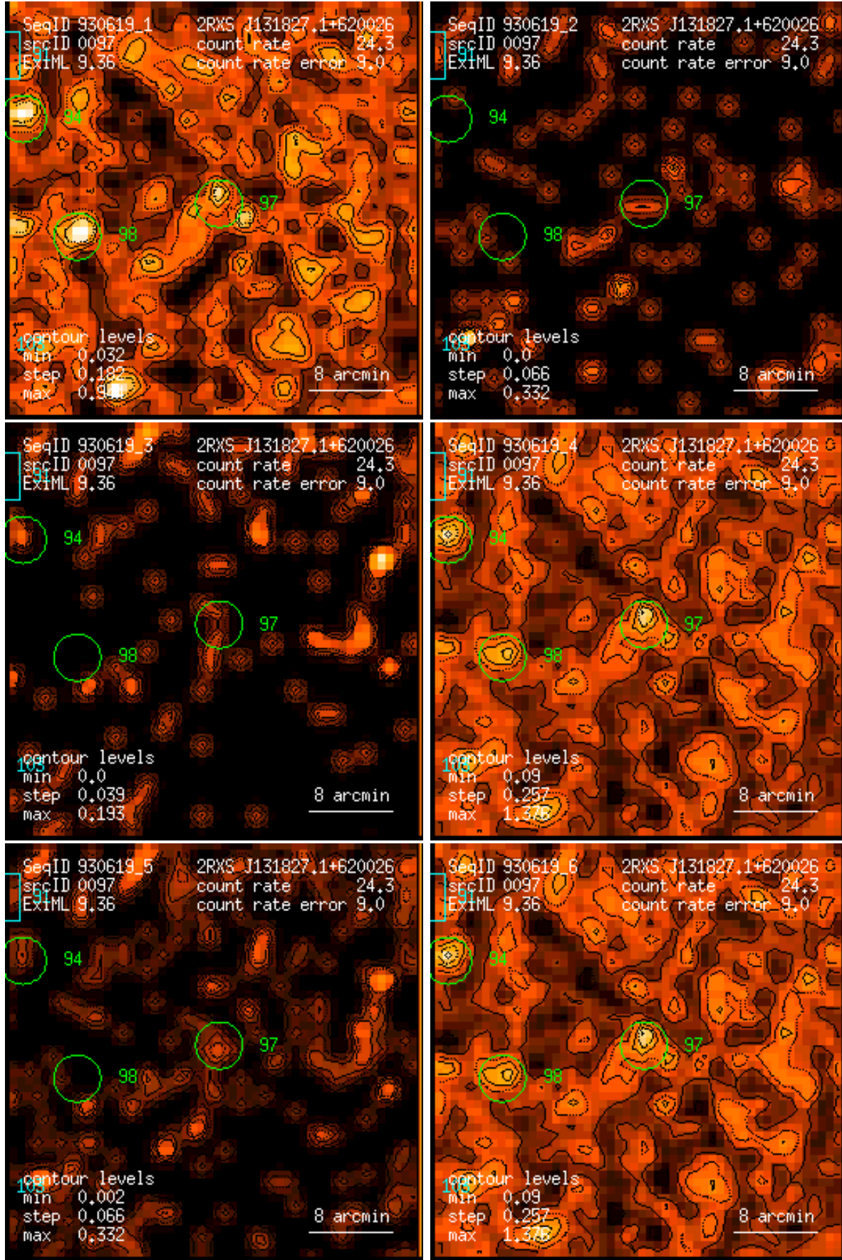
Figure 97: RASS 930619: detection 0097: band rate images, Gaussian filter: (1) PSPC channels 11 – 41, (2) 52 – 90, (3) 91 – 201, (4) 11 – 235, (5) 52 – 201, (6) 11 – 201. Broad band rates in counts/ks. Band rate contour levels in counts/ks/arcmin 2 .
