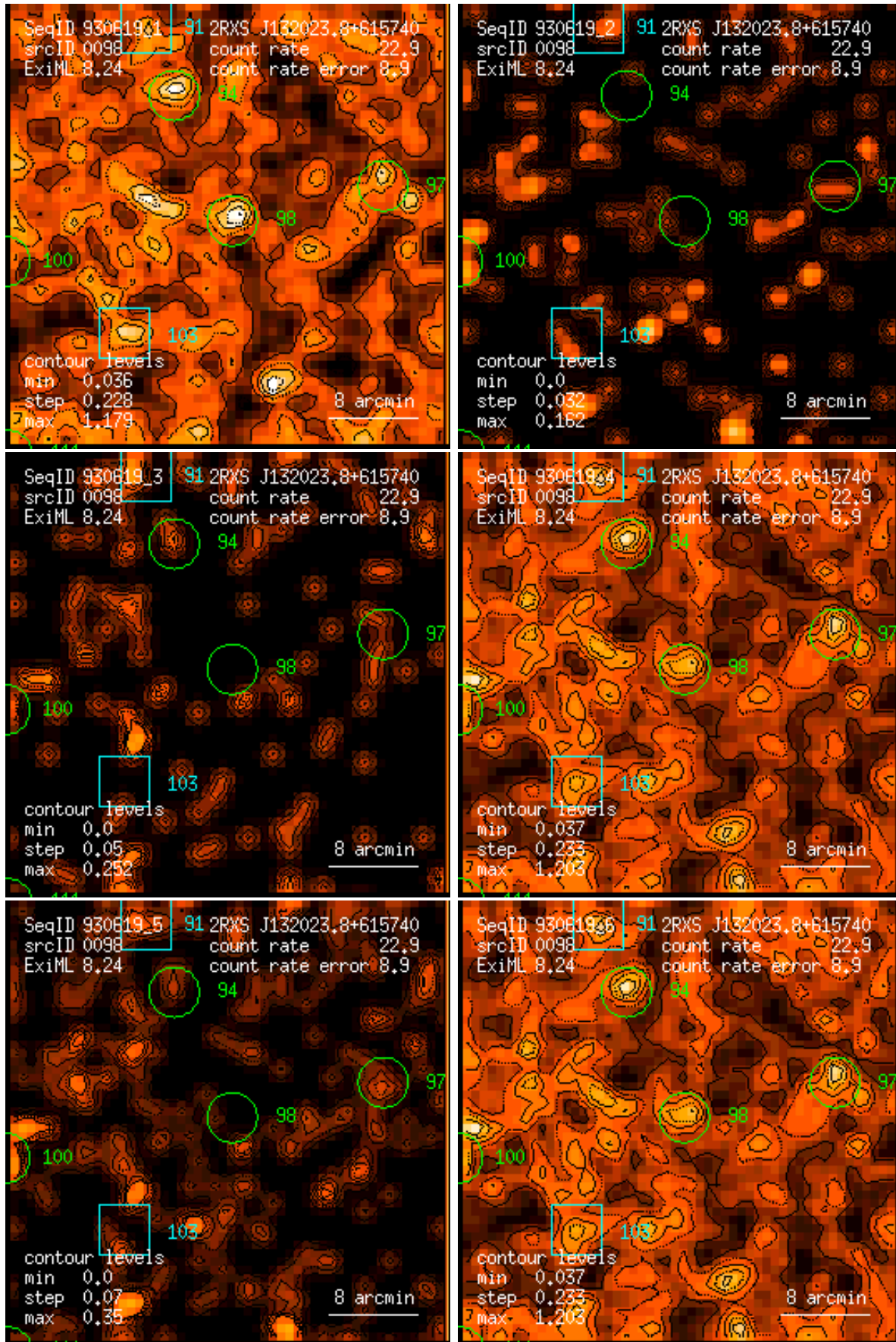
Figure 98: RASS 930619: detection 0098: band rate images, Gaussian filter: (1) PSPC channels 11 – 41, (2) 52 – 90, (3) 91 – 201, (4) 11 – 235, (5) 52 – 201, (6) 11 – 201. Broad band rates in counts/ks. Band rate contour levels in counts/ks/arcmin 2 .
