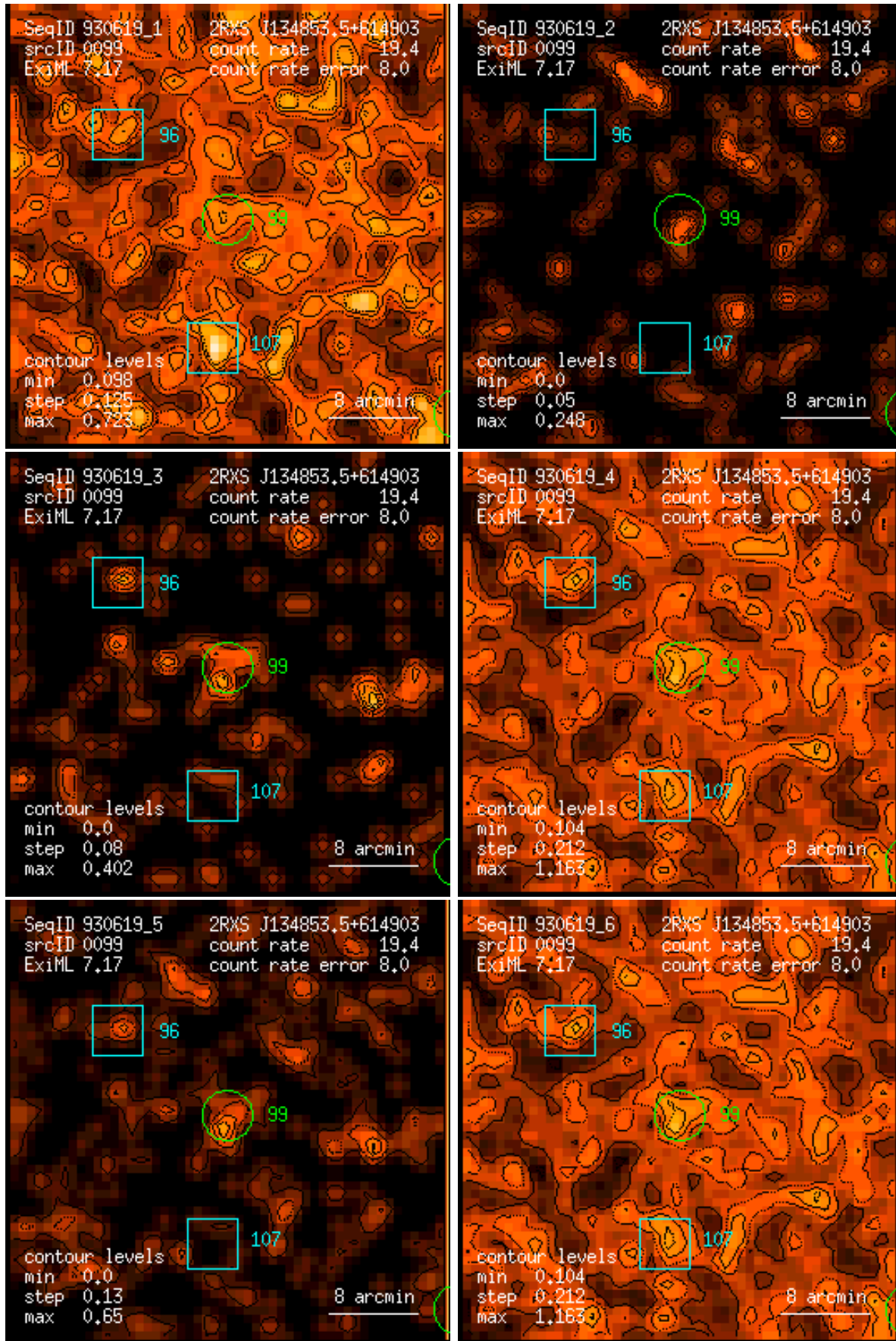
Figure 99: RASS 930619: detection 0099: band rate images, Gaussian filter: (1) PSPC channels 11 – 41, (2) 52 – 90, (3) 91 – 201, (4) 11 – 235, (5) 52 – 201, (6) 11 – 201. Broad band rates in counts/ks. Band rate contour levels in counts/ks/arcmin 2 .
