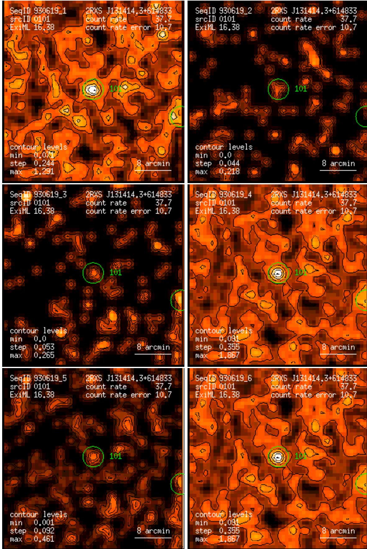
Figure 101: RASS 930619: detection 0101: band rate images, Gaussian filter: (1) PSPC channels 11 – 41, (2) 52 – 90, (3) 91 – 201, (4) 11 – 235, (5) 52 – 201, (6) 11 – 201. Broad band rates in counts/ks. Band rate contour levels in counts/ks/arcmin 2 .
