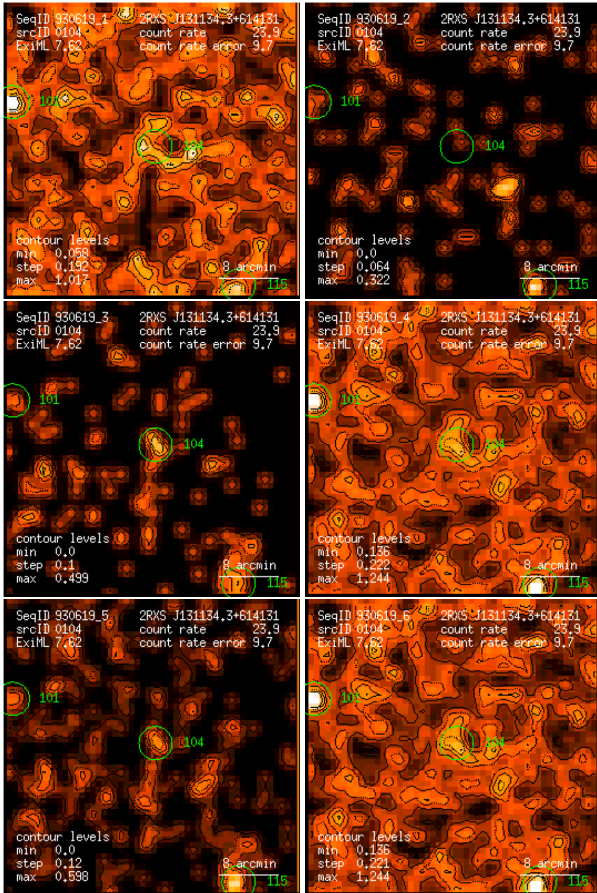
Figure 104: RASS 930619: detection 0104: band rate images, Gaussian filter: (1) PSPC channels 11 – 41, (2) 52 – 90, (3) 91 – 201, (4) 11 – 235, (5) 52 – 201, (6) 11 – 201. Broad band rates in counts/ks. Band rate contour levels in counts/ks/arcmin 2 .
