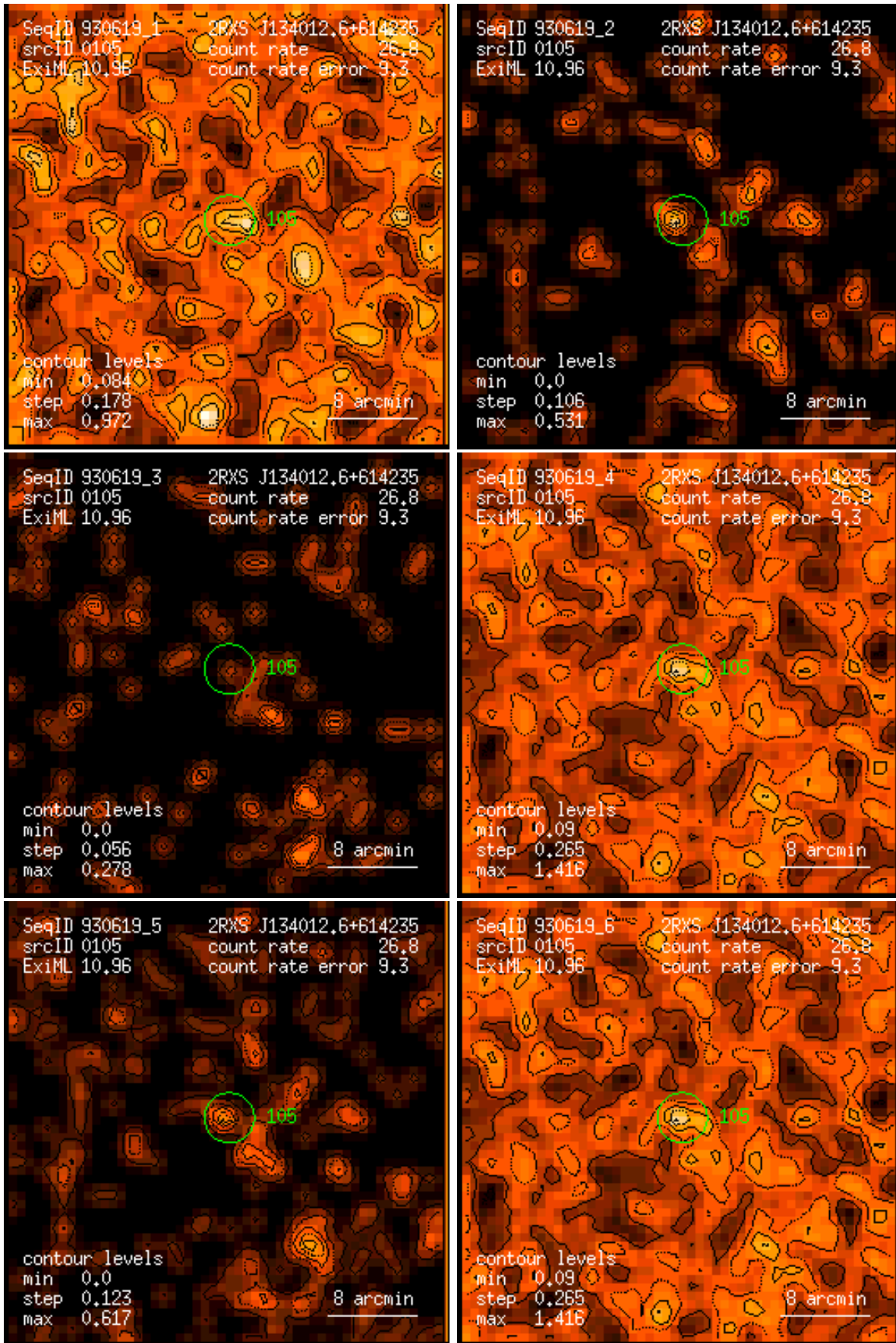
Figure 105: RASS 930619: detection 0105: band rate images, Gaussian filter: (1) PSPC channels 11 – 41, (2) 52 – 90, (3) 91 – 201, (4) 11 – 235, (5) 52 – 201, (6) 11 – 201. Broad band rates in counts/ks. Band rate contour levels in counts/ks/arcmin 2 .
