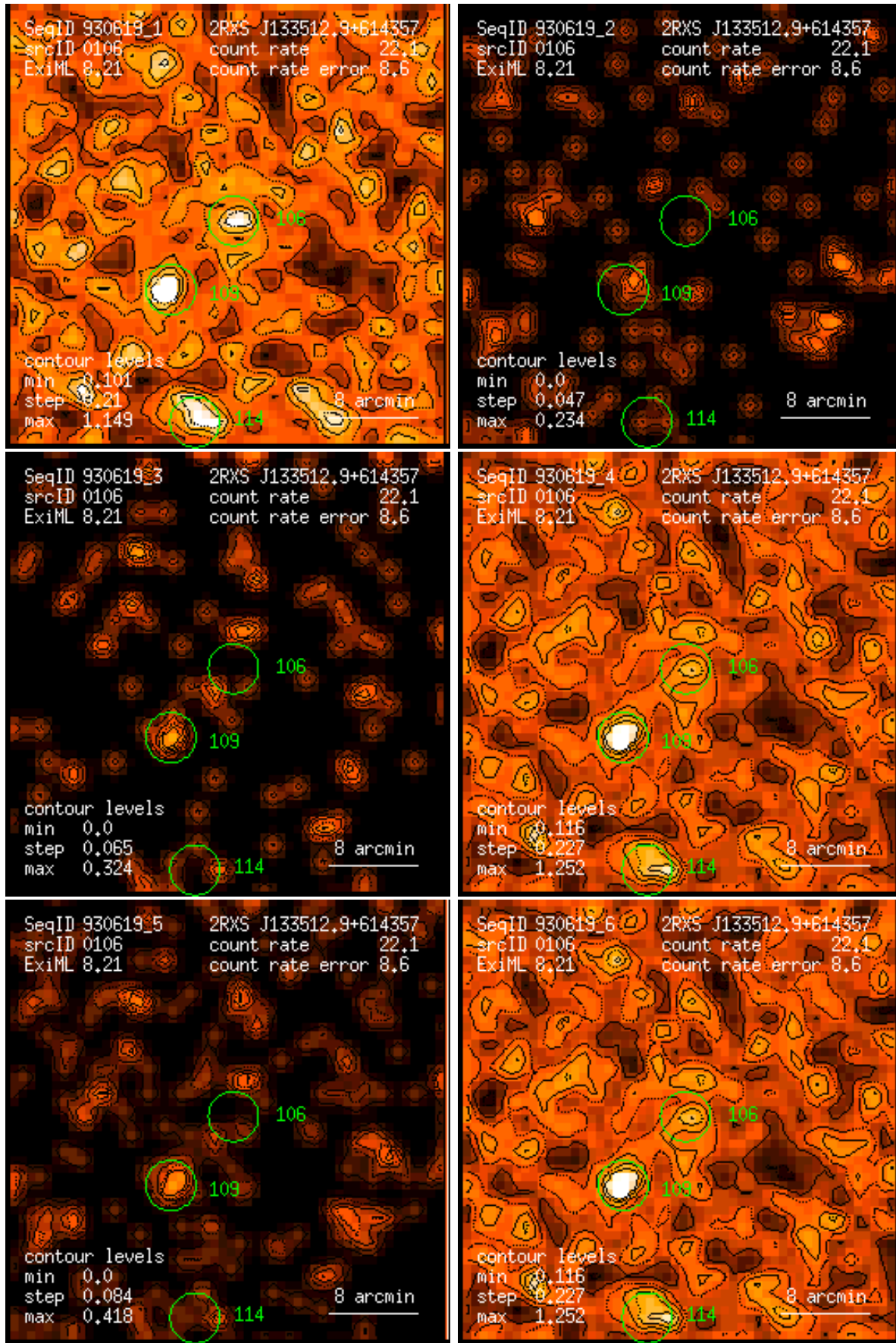
Figure 106: RASS 930619: detection 0106: band rate images, Gaussian filter: (1) PSPC channels 11 – 41, (2) 52 – 90, (3) 91 – 201, (4) 11 – 235, (5) 52 – 201, (6) 11 – 201. Broad band rates in counts/ks. Band rate contour levels in counts/ks/arcmin 2 .
