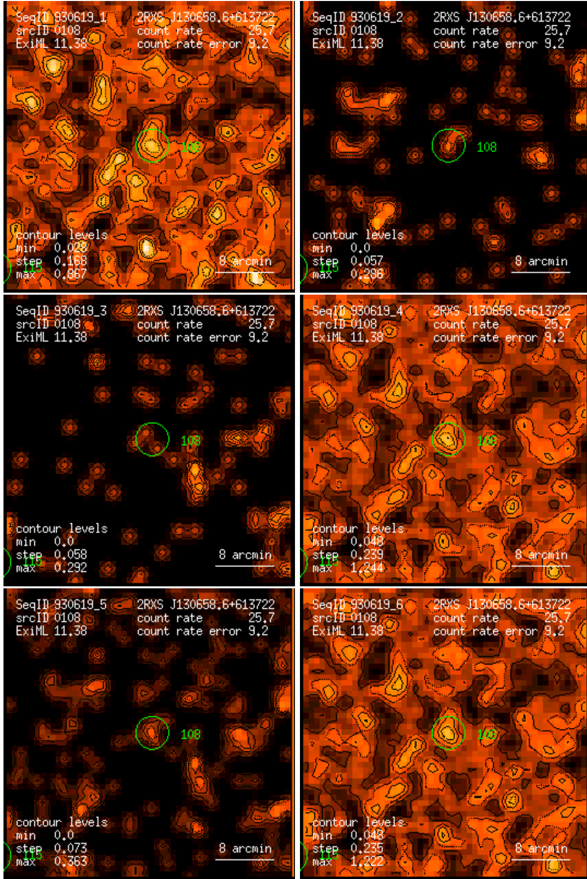
Figure 108: RASS 930619: detection 0108: band rate images, Gaussian filter: (1) PSPC channels 11 – 41, (2) 52 – 90, (3) 91 – 201, (4) 11 – 235, (5) 52 – 201, (6) 11 – 201. Broad band rates in counts/ks. Band rate contour levels in counts/ks/arcmin 2 .
