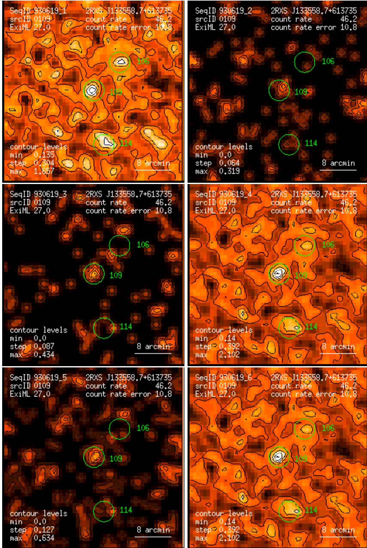
Figure 109: RASS 930619: detection 0109: band rate images, Gaussian filter: (1) PSPPC channels 11 – 41, (2) 52 – 90, (3) 91 – 201, (4) 11 – 235, (5) 52 – 201, (6) 11 – 201. Broad band rates in counts/ks. Band rate contour levels in counts/ks/arcmin 2 .
